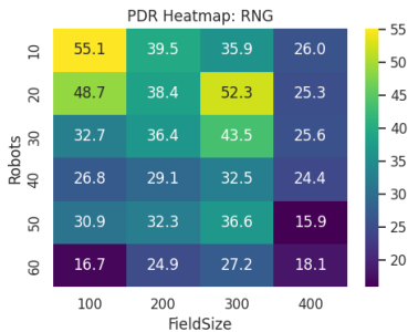
Figure 3.7: RNG multi-hop PDR heatmap across network scales and deployment areas. Shows consistent performance with graceful degradation, reaching 55.1% peak PDR in multi-hop routing scenarios.
