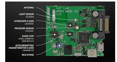
Figure 5.1: The IoT-LAB M3 board [131]
