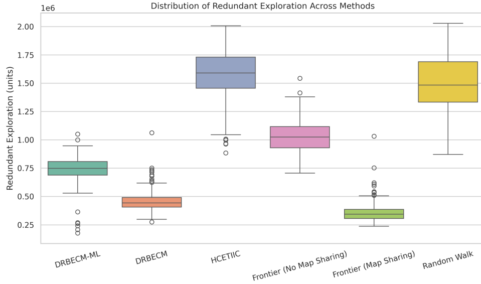
Figure 5.5: Comparison of redundant exploration across the different methods.
