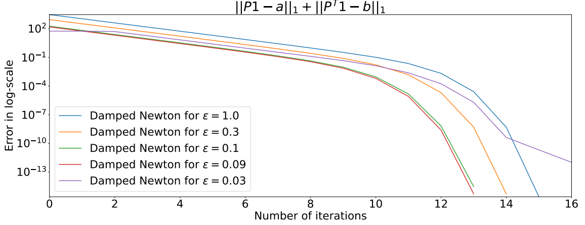
FIGURE 6.3.7. Convergence speed of damped Newton. This illustration shows that the algorithm converges with much fewer steps, in a way that is insensitive to \varepsilon > 0 .
