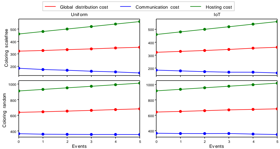
Figure 6.25 – Cost of the distribution of computation graphs on which A-MaxSum operates, after each event, on uniform (left) and problem-dependent (right) infrastructure, and when solving scale free graph coloring (top) and random graph coloring (bottom) problems, using DRPM[MGM-2] to repair
