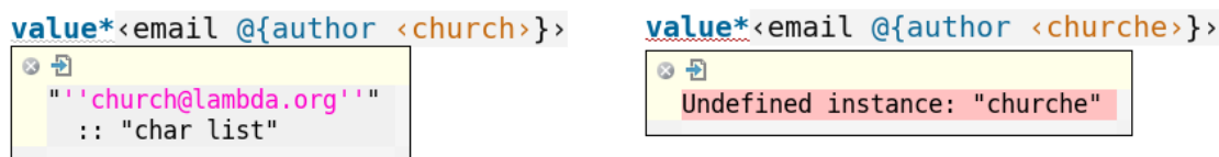
Figure 3.3: Evaluation of Antiquotations in a Term-Context.
