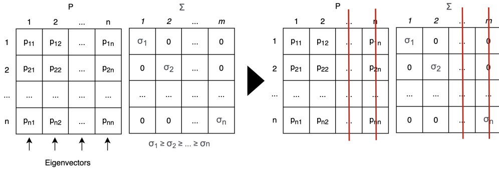
Figure 4.4: Discarding the smallest eigenvalues and corresponding eigenvectors in SVD.
