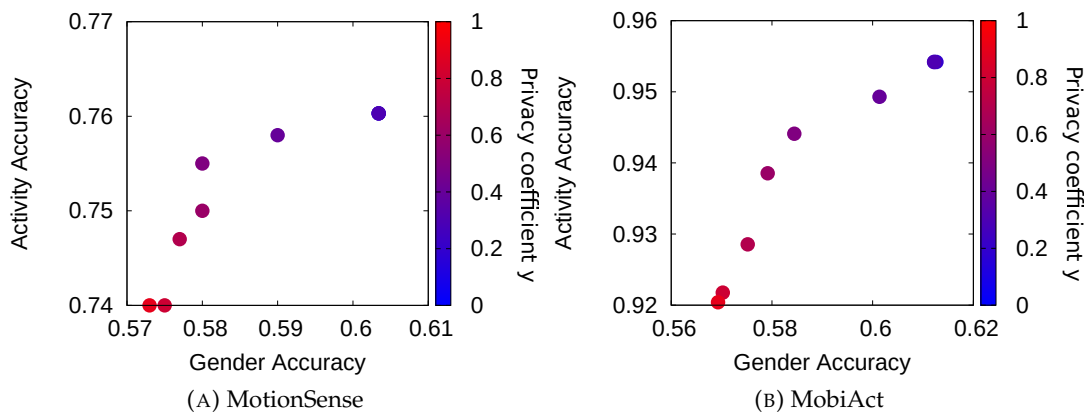
FIGURE IV.4 – The variation of the Privacy coefficient y from 0.1 to 0.9 implies a variation of the trade-off between Utility and Privacy.
