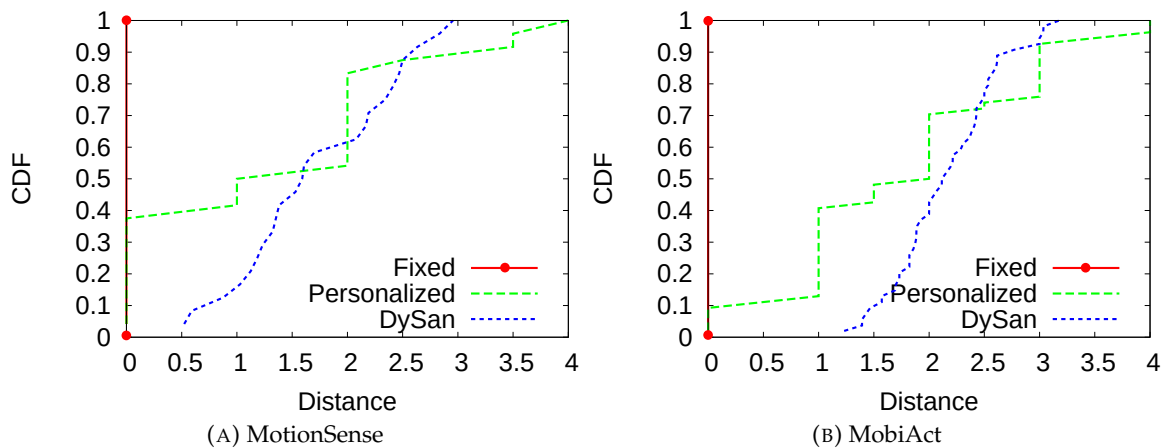
FIGURE IV.9 – DYSAN provides a large variability in terms of distance over all users highlighting the necessity to provide a variety of models to adapt the sanitization.
