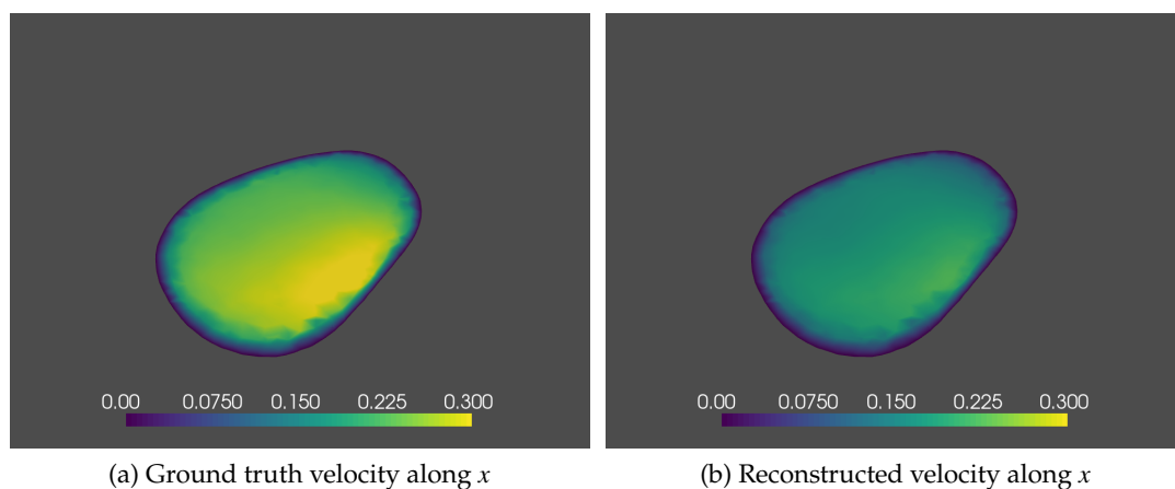
Figure 1.15: The non-stationary velocity field along x for z = 0.155 and t = 0.05\text{s} , for a PPSNR = 40 dB.
