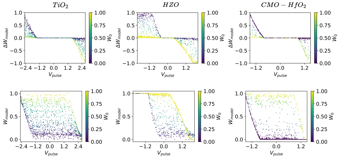
Supplementary Fig. 4.1 The fitted model's prediction on characterization data points displays the weight change ( \Delta W ) and final weight ( W_f ) in relation to the applied voltage ( V_{pulse} ) and initial weight ( W_0 ) for TiO_2 , HZO , and CMO-HfO_2 measurement points (from left to right).
