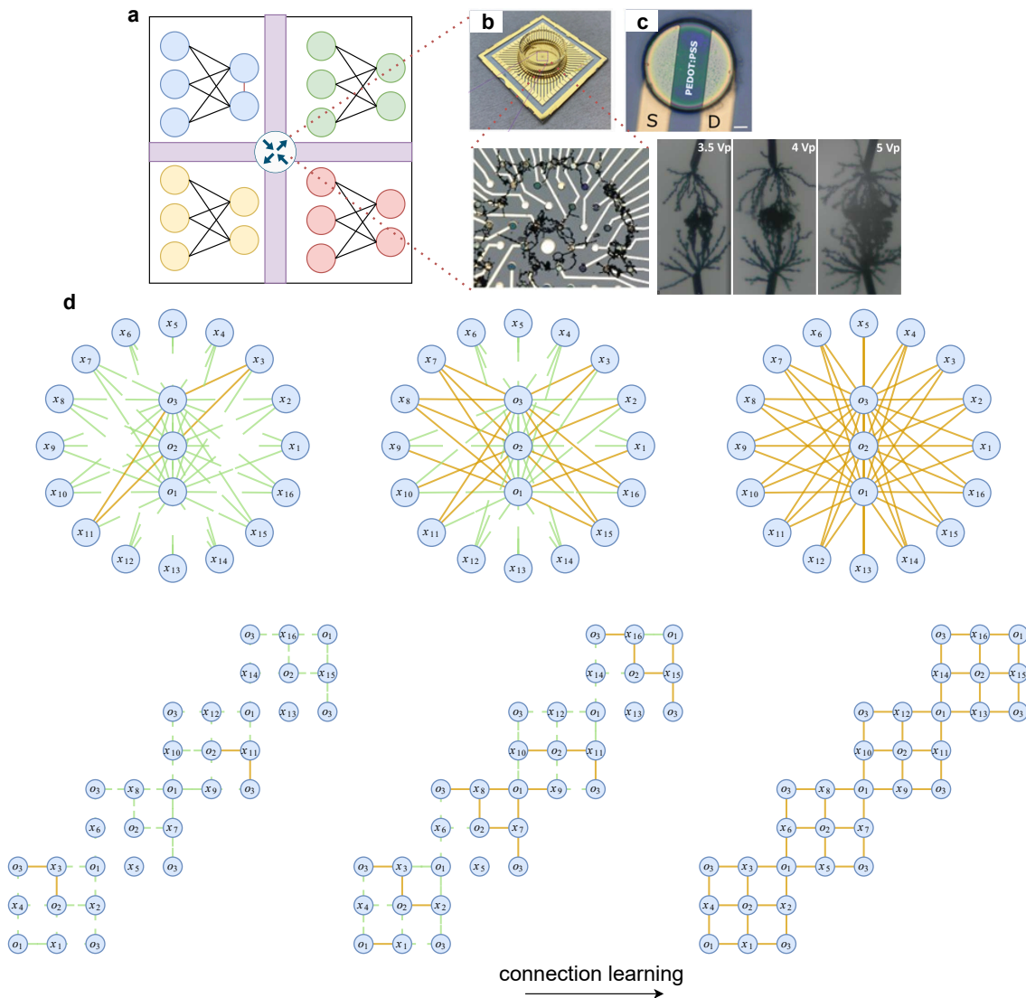
Figure 7.1 Multi-core architecture with plastic interconnects. (Adapted with permission from [290]) a Multicore architecture composed of multiple CMOS-RRAM neural building blocks, interconnected by a programmable router. b The programmable router consists of an array of Organic Electrochemical Transistor (OECT)s (top). 2D microelectrode arrays with dendritic connections (bottom). c Between the source and drain, there is a PEDOT:PSS polymer (top), which transforms into conducting interconnects upon electrical stimulation (bottom). d In a hardware-mapped 3D network, through learning connections with structural plasticity, each node connects to its nearest neighbors.
