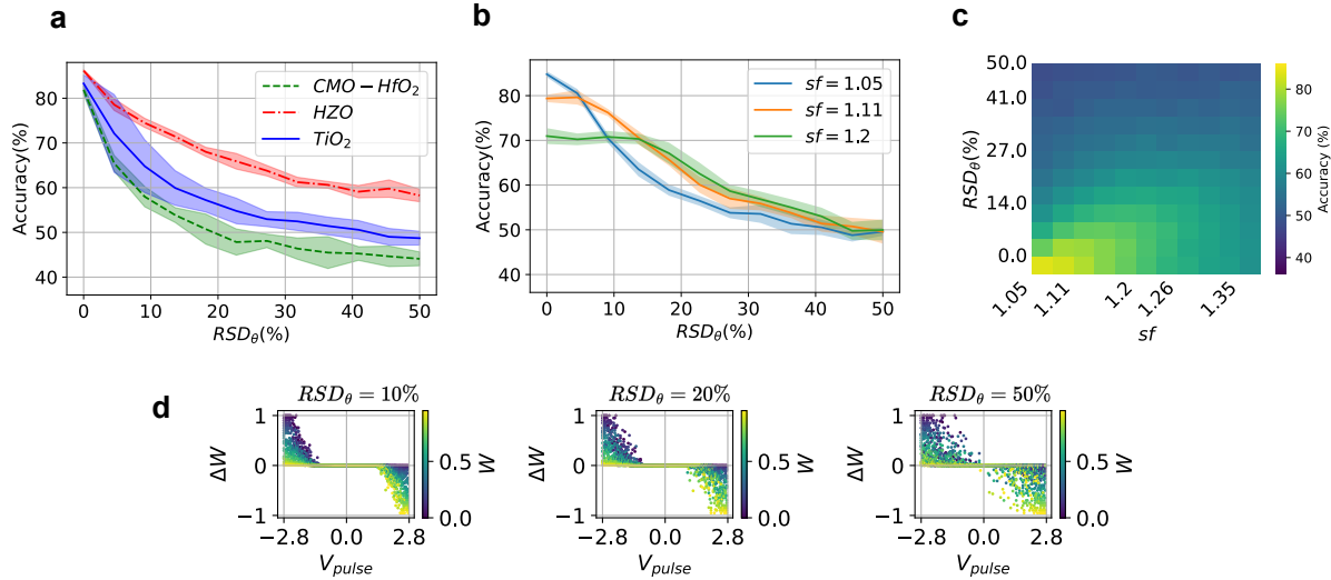
Figure 4.6 Impact of device-to-device variability in switching threshold. a The switching thresholds ( \theta ) for the 784x200 synapses are sampled from a normal distribution centered on the fitted model parameter. The relative standard dispersion, represented as \frac{\sigma}{\mu} , varies and is noted as RSD_{\theta} . b The resulting accuracy is shown for three distinct values of sf for TiO_2 device parameters. (Note that the other two devices follow a similar trend, as illustrated in Supplementary Figure 4.4 and Supplementary Figure 4.5. c A detailed grid search of sf and RSD_{\theta} was conducted, and the resulting average accuracy over ten experiments is displayed as a 2-D heatmap. d Plots of device characteristics depicting \Delta W versus V_{pulse} to demonstrate the variability effects for three \frac{\sigma}{\mu} levels: 0.1, 0.2, and 0.5 (arranged from left to right).
