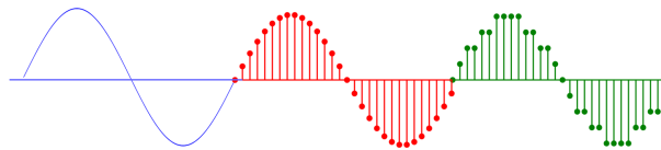
Figure 2.5 Analog to digital domain conversion. Natural signals are analog, and are continuous in amplitude and time. These are captured at regular time intervals to create sampled signals. Thereafter, the amplitude of the signals is quantized to produce digital signals for storage and processing.
