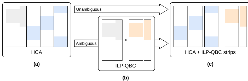
Fig. 3 Hybrid strip search HCA + ILP-QBC. In each of the sub-figure, the colored areas are dense binary sub-matrices. (a) The initial matrix with the groups of columns found via HCA. The first one (grey areas) is not a strip, as the bipartitioning does not respect \gamma . The other three (blue tiles) are strips. (b) The remaining matrix is sent to ILP-QBC to find strips respecting \gamma . In this example, ILP-QBC finds two strips (orange tiles). (c) The final set of strips is composed of the HCA-based strips and the ones found by ILP-QBC.
