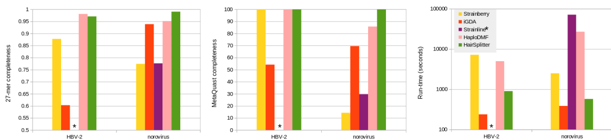
Figure 5. 27-mer completeness, MetaQUAST completeness and run-time of different software on the two viral datasets. Note that the run-time is shown in log scale. The Strainline assembly of HBV-2 is not shown because Strainline could not finish on this dataset.
