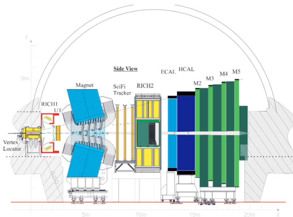
Figure 3.28: Cross section of the upgraded LHCb detector [148]
