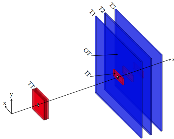
Figure 3.11: Layout of the tracking system [111]
