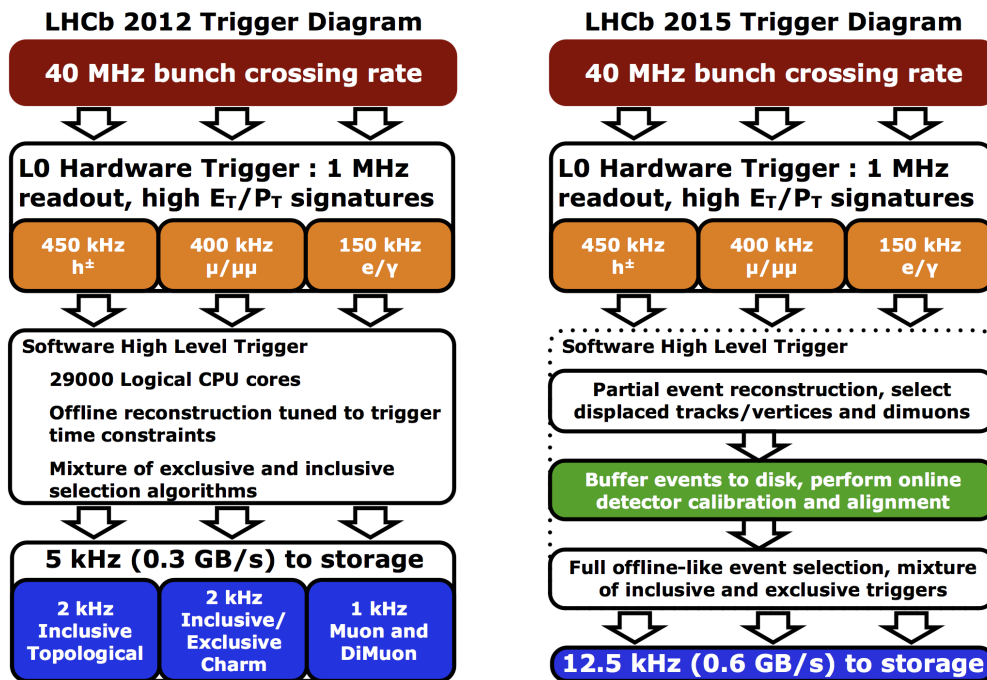
Figure 3.24: Left: Trigger scheme in Run 1. Right: Trigger scheme in Run 2 [136].
