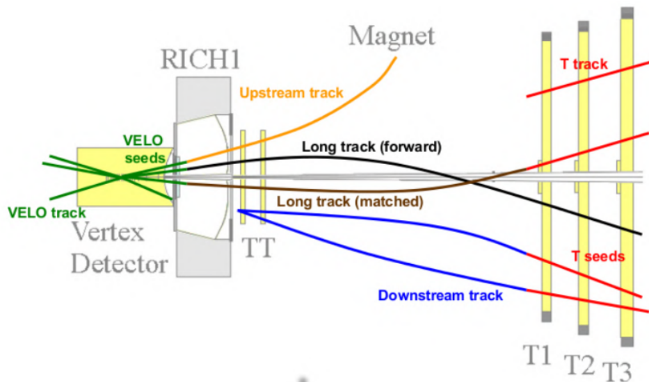
Figure 3.14: Different track types reconstructed at LHCb [114]
