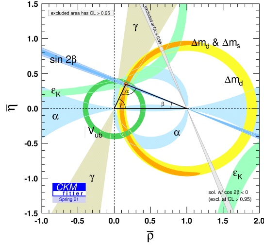
Figure 2.5: Measurements of the CKM unitarity triangle as of spring 2021. [43]
