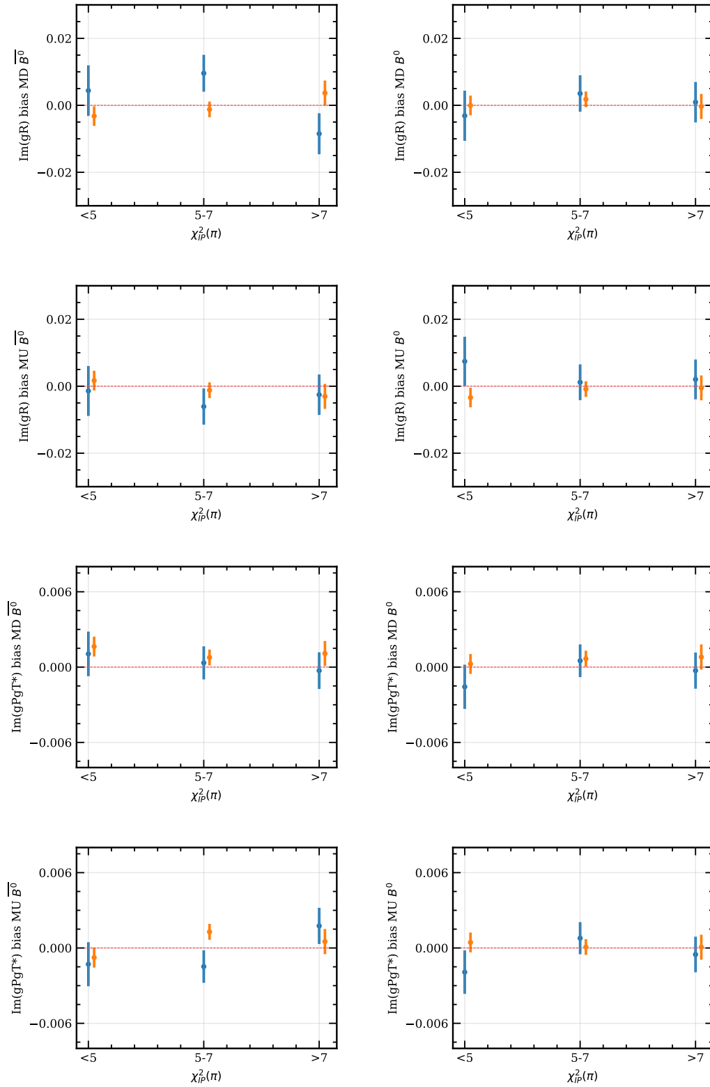
Figure 35: NP couplings bias for signal (orange) and control (blue) samples in bins of \chi_{IP}^2(\pi) across the four categories
