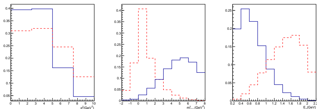
Figure 4.12: Projections of the 3D template in q^2 , m_{miss}^2 and E_\mu^* for the B^+ \rightarrow D^{*-} D_{(s)}^+ X, D_{(s)}^+ \rightarrow X \mu^+ \nu_\mu sample in blue. The signal projections are shown in red for comparison.
