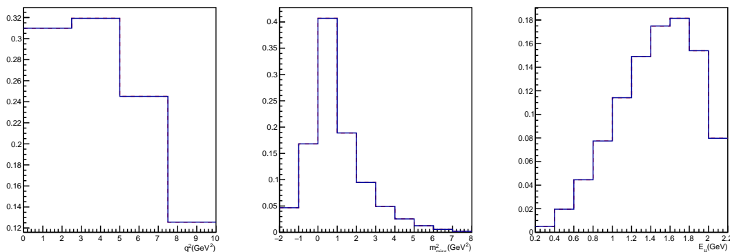
Figure 4.7: Projections of the 3D template in q^2 , m_{\text{miss}}^2 and E_\mu^* for the B^0 \rightarrow D^{*-} \mu^+ \nu_\mu signal sample
