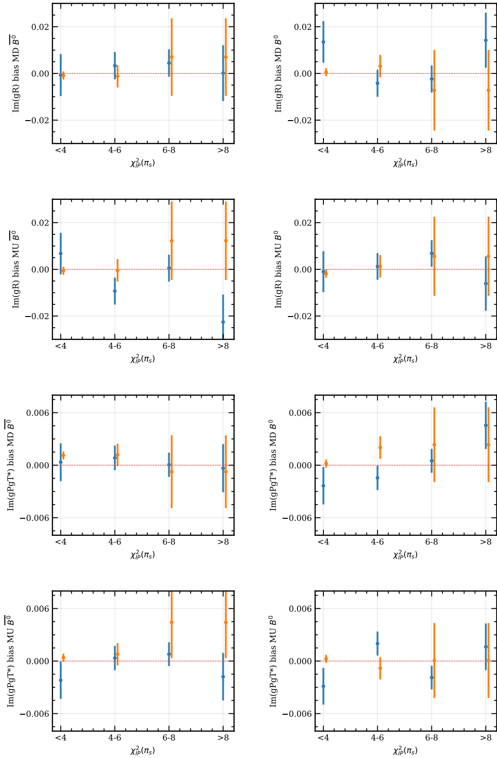
Figure 38: NP couplings bias for signal (orange) and control (blue) samples in bins of \chi_{\text{IP}}^2(\pi_s) across the four categories
