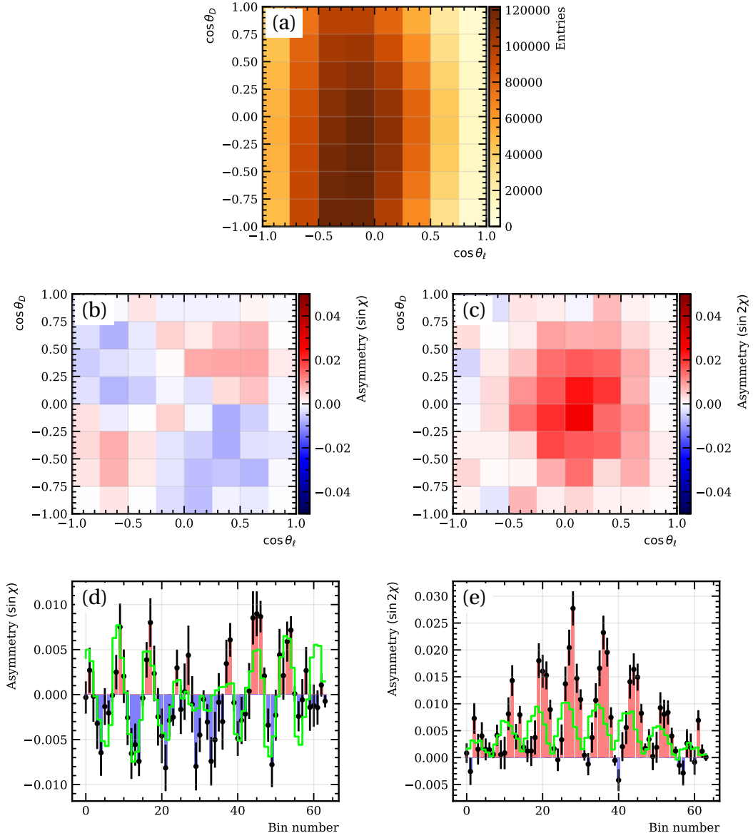
Figure 4.24: Binned density (a), binned 2D parity asymmetries (b,c) and flattened 1D parity asymmetries (d,e) of \sin \chi and \sin 2\chi terms in (\cos \theta_D, \cos \theta_\ell) bins integrated over q^2 for the B^+ \rightarrow D^{**0} \mu^+ \nu_\mu simulation sample with strong phase \delta_D = 315^\circ . Figures (d) and (e) also show the result of the best fit in green using the RH and PT templates.
