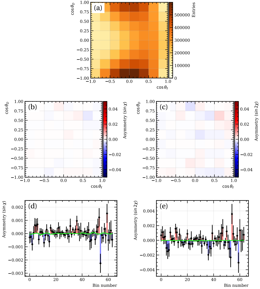
Figure 4.36: Binned density (a), binned 2D parity asymmetries (b,c) and flattened 1D parity asymmetries (d,e) of \sin \chi and \sin 2\chi terms in (\cos \theta_D, \cos \theta_\ell) bins integrated over q^2 for the T_y misalignment B^0 \rightarrow D^{*-} \mu^+ \nu_\mu simulation sample. Figures (d) and (e) also show the result of the best fit in green using the RH and PT templates.
