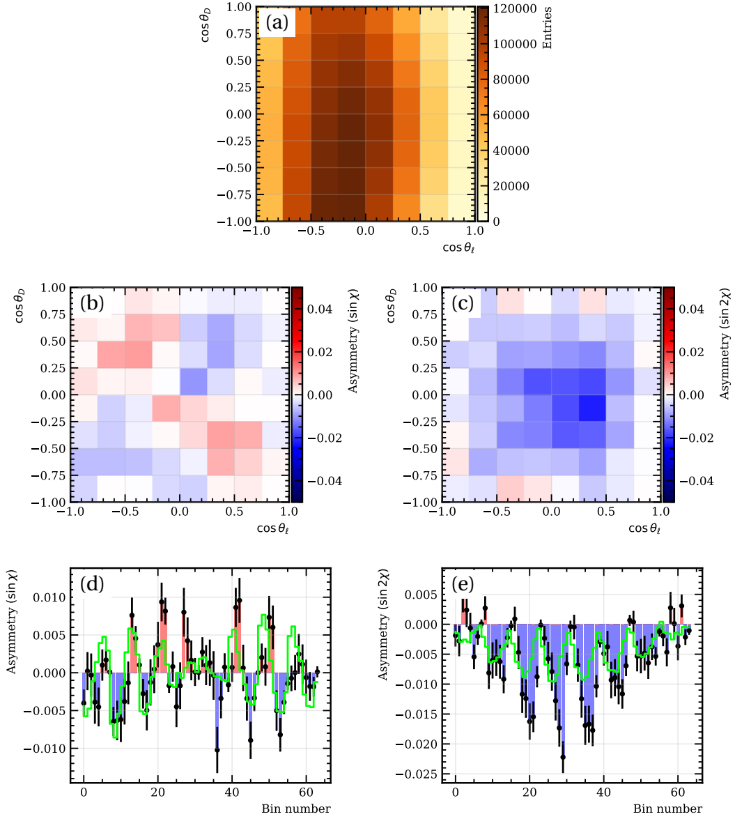
Figure 3: Binned density (a), binned 2D parity asymmetries (b,c) and flattened 1D parity asymmetries (d,e) of \sin \chi and \sin 2\chi terms in (\cos \theta_D, \cos \theta_\ell) bins integrated over q^2 for the B^+ \rightarrow D^{*0} \mu^+ \nu_\mu with \delta_D = 90^\circ . Figures (d) and (e) also show the result of the best fit in green using the RH and PT templates.
