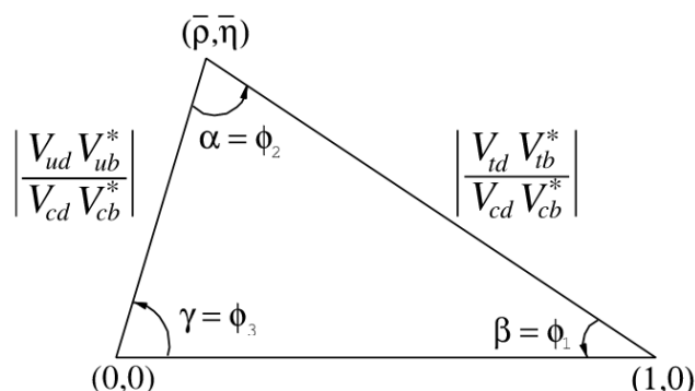
Figure 2.4: The unitarity triangle shown in the complex plane [45].
