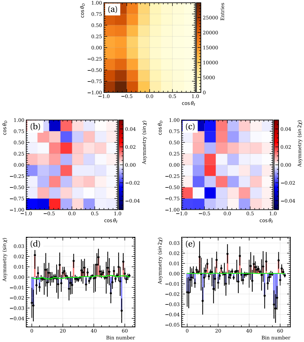
Figure 4.26: Binned density (a), binned 2D parity asymmetries (b,c) and flattened 1D parity asymmetries (d,e) of \sin\chi and \sin 2\chi terms in (\cos\theta_D, \cos\theta_\ell) bins integrated over q^2 for the weighted B^0 \rightarrow D^{*-} D_s^{*+} simulation sample (maximal parity violation). Figures (d) and (e) also show the result of the best fit in green using the RH and PT templates.
