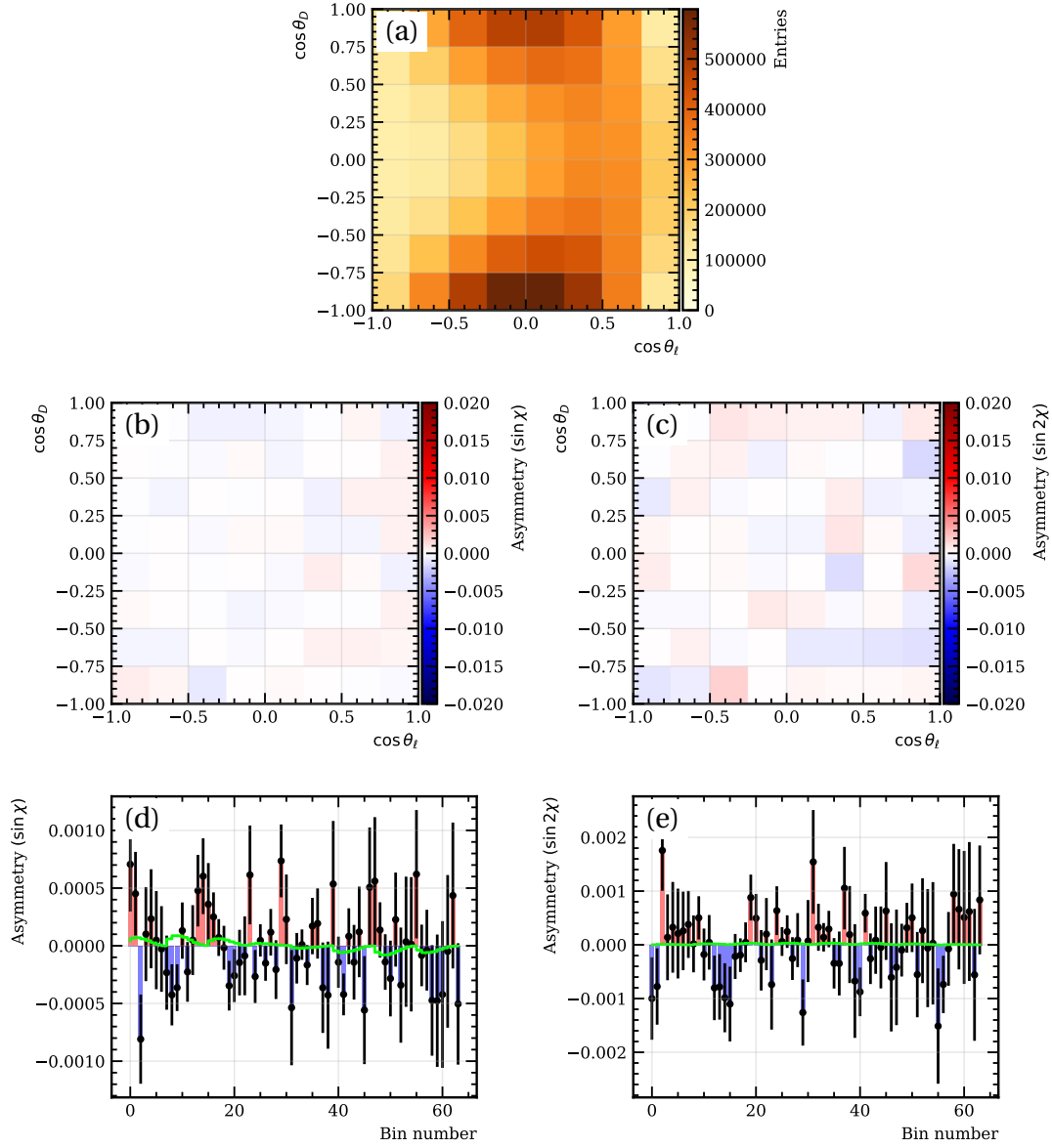
Figure 10: Binned density (a), binned 2D CP asymmetries (b,c) and flattened 1D CP asymmetries (d,e) of \sin\chi and \sin 2\chi terms in (\cos\theta_D, \cos\theta_\ell) bins integrated over q^2 for the T_z misalignment sample. Figures (d) and (e) also show the result of the best fit in green using the RH and PT templates.
