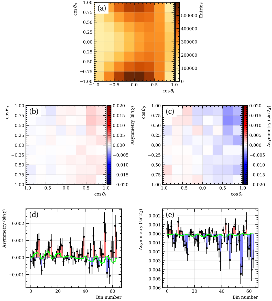
Figure 16: Binned density (a), binned 2D CP asymmetries (b,c) and flattened 1D CP asymmetries (d,e) of \sin\chi and \sin 2\chi terms in (\cos\theta_D, \cos\theta_\ell) bins integrated over q^2 for the R_z misalignment sample. Figures (d) and (e) also show the result of the best fit in green using the RH and PT templates.
