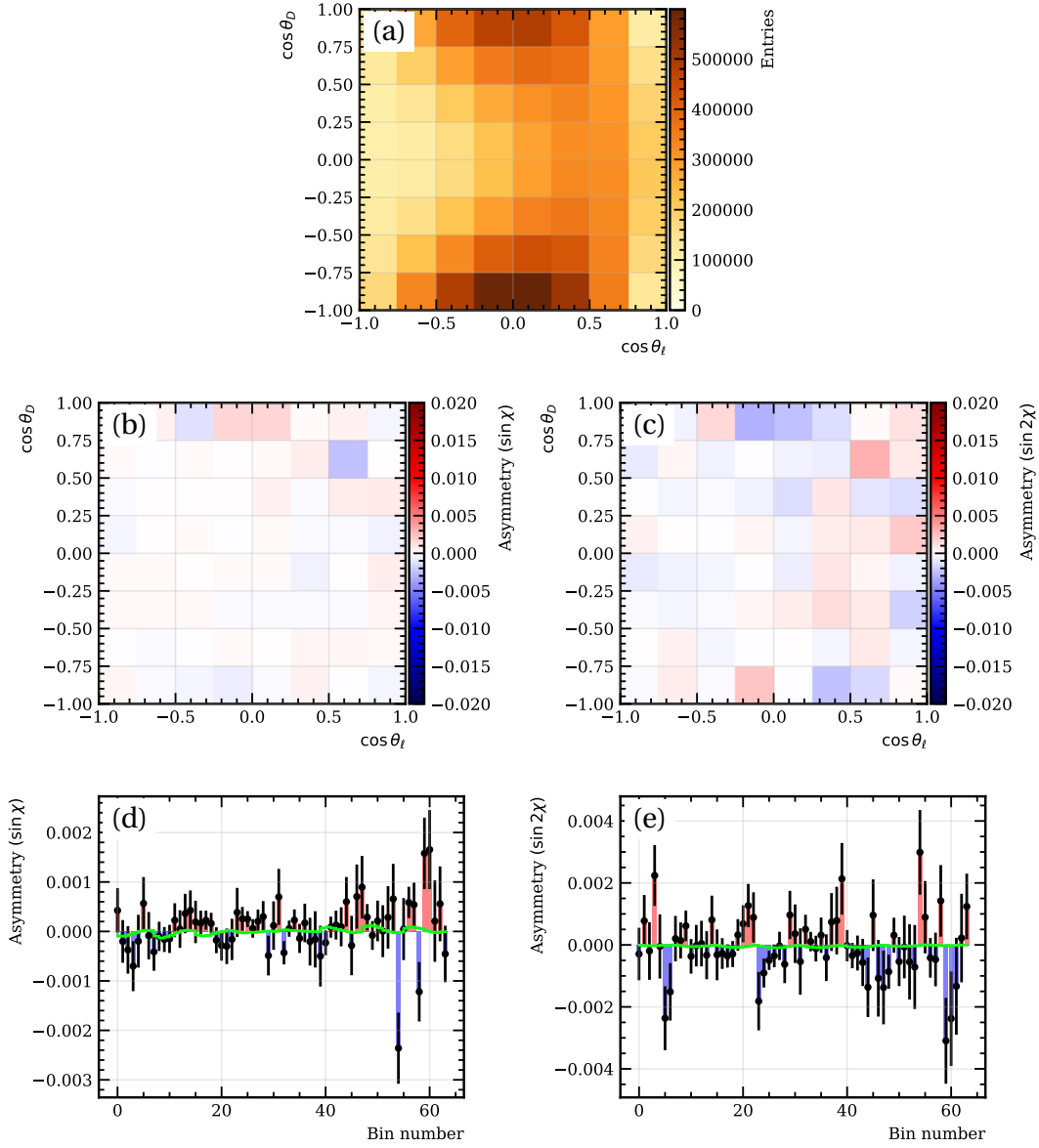
Figure 9: Binned density (a), binned 2D parity asymmetries (b,c) and flattened 1D parity asymmetries (d,e) of \sin \chi and \sin 2\chi terms in (\cos \theta_D, \cos \theta_\ell) bins integrated over q^2 for the T_x misalignment sample. Figures (d) and (e) also show the result of the best fit in green using the RH and PT templates.
