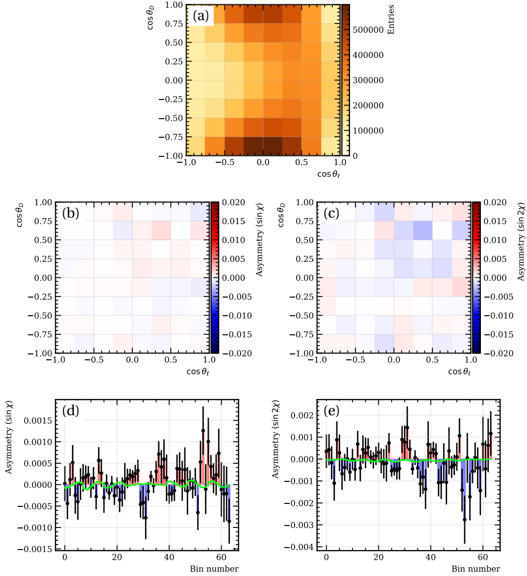
Figure 11: Binned density (a), binned 2D parity asymmetries (b,c) and flattened 1D parity asymmetries (d,e) of \sin \chi and \sin 2\chi terms in (\cos \theta_D, \cos \theta_\ell) bins integrated over q^2 for the T_z misalignment sample. Figures (d) and (e) also show the result of the best fit in green using the RH and PT templates.
