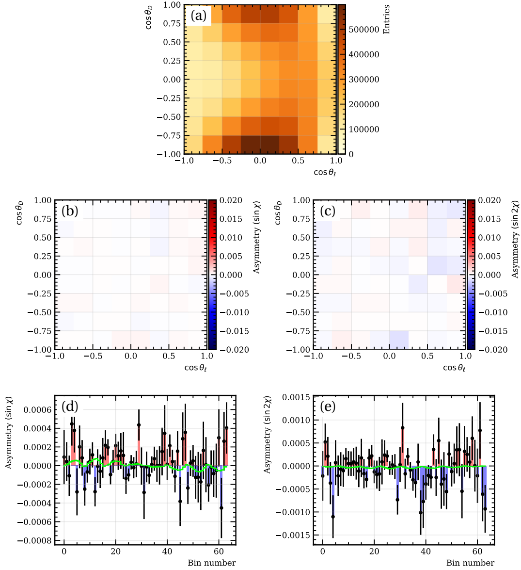
Figure 14: Binned density (a), binned 2D CP asymmetries (b,c) and flattened 1D CP asymmetries (d,e) of \sin \chi and \sin 2\chi terms in (\cos \theta_D, \cos \theta_\ell) bins integrated over q^2 for the R_\gamma misalignment sample. Figures (d) and (e) also show the result of the best fit in green using the RH and PT templates.
