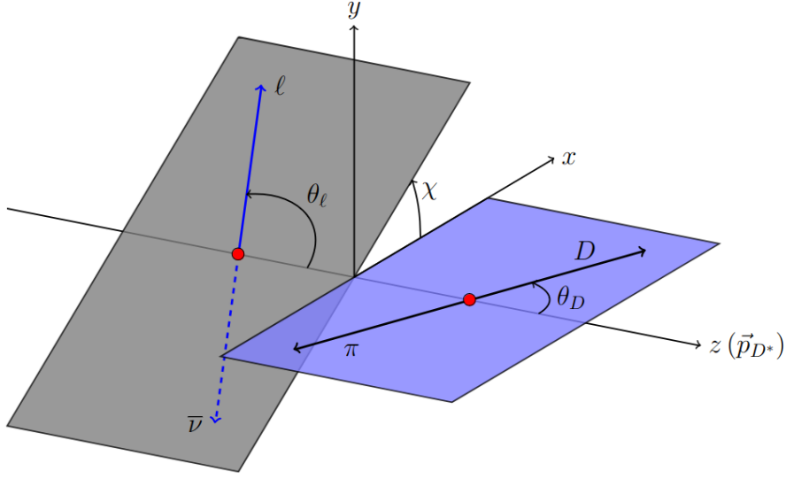
Figure 2.15: Helicity angles of the \bar{B} \rightarrow D^* (\rightarrow D\pi)\ell\bar{\nu}_\ell decay. Figure taken from [3].
