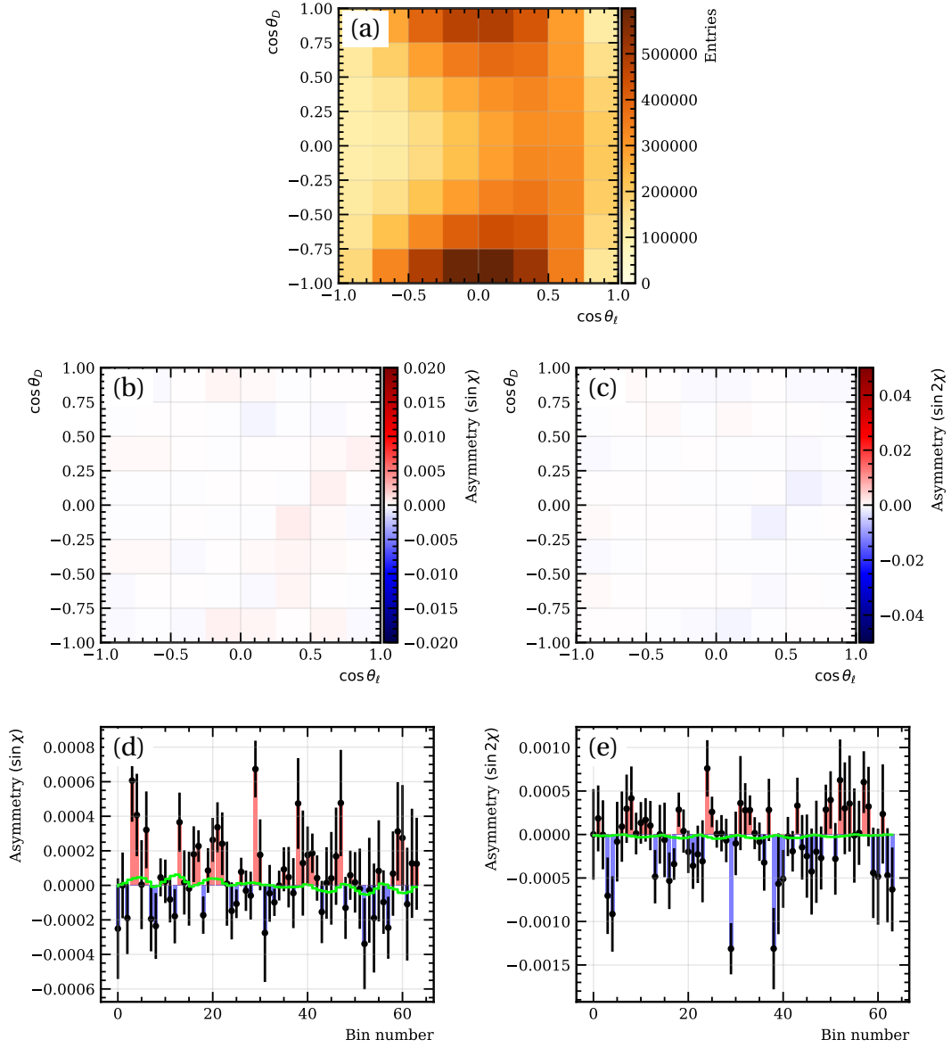
Figure 12: Binned density (a), binned 2D CP asymmetries (b,c) and flattened 1D CP asymmetries (d,e) of \sin\chi and \sin 2\chi terms in (\cos\theta_D, \cos\theta_\ell) bins integrated over q^2 for the R_x misalignment sample. Figures (d) and (e) also show the result of the best fit in green using the RH and PT templates.
