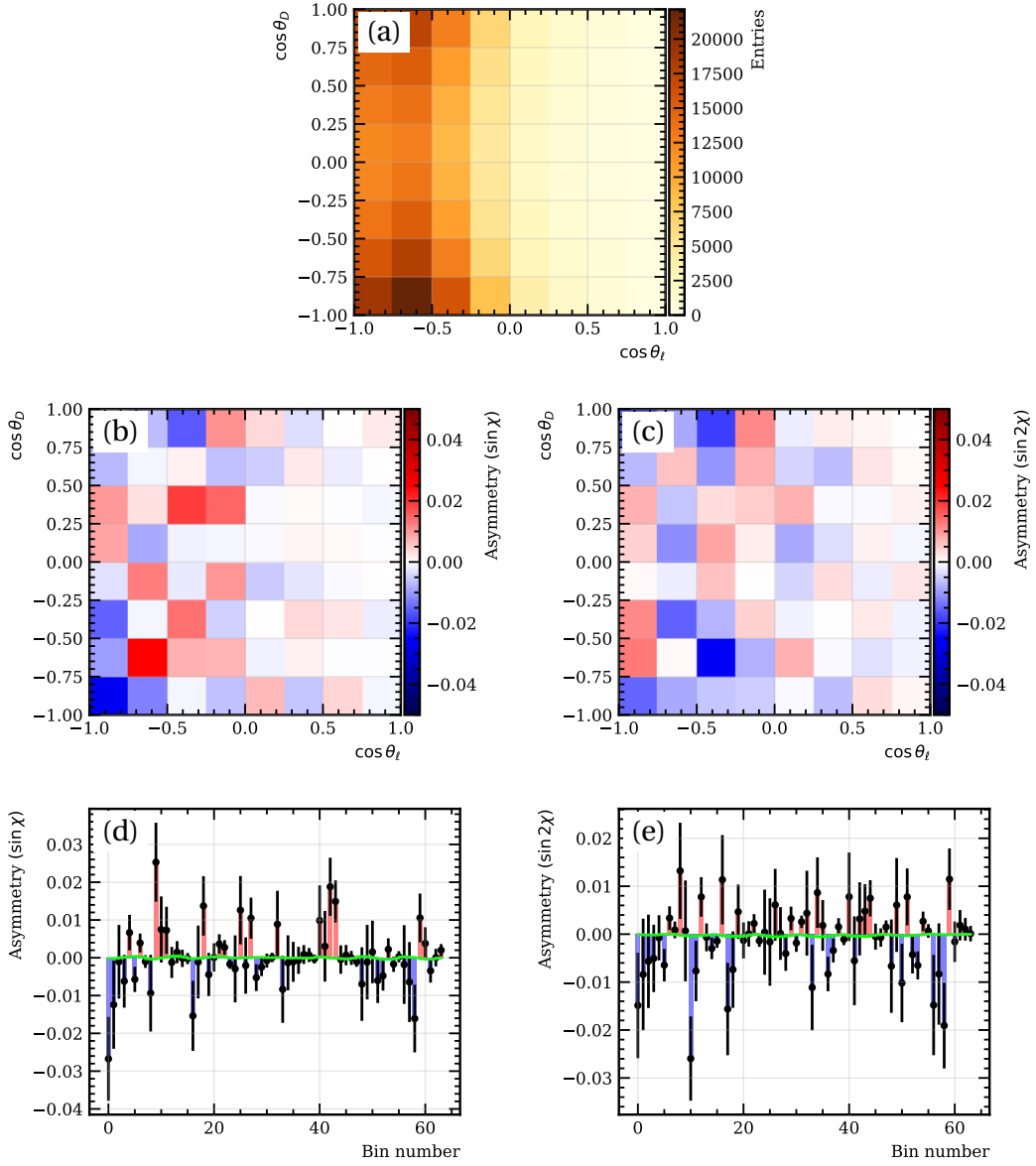
Figure 4.25: Binned density (a), binned 2D parity asymmetries (b,c) and flattened 1D parity asymmetries (d,e) of \sin \chi and \sin 2\chi terms in (\cos \theta_D, \cos \theta_\ell) bins integrated over q^2 for the unweighted B^0 \rightarrow D^{*-} D_s^{*+} simulation sample (no parity violation). Figures (d) and (e) also show the result of the best fit in green using the RH and PT templates.
