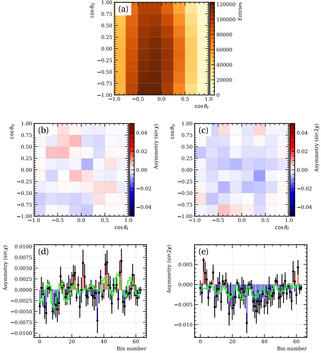
Figure 2: Binned density (a), binned 2D parity asymmetries (b,c) and flattened 1D parity asymmetries (d,e) of \sin \chi and \sin 2\chi terms in (\cos \theta_D, \cos \theta_\ell) bins integrated over q^2 for the B^+ \rightarrow D^{*0} \mu^+ \nu_\mu with \delta_D = 45^\circ . Figures (d) and (e) also show the result of the best fit in green using the RH and PT templates.
