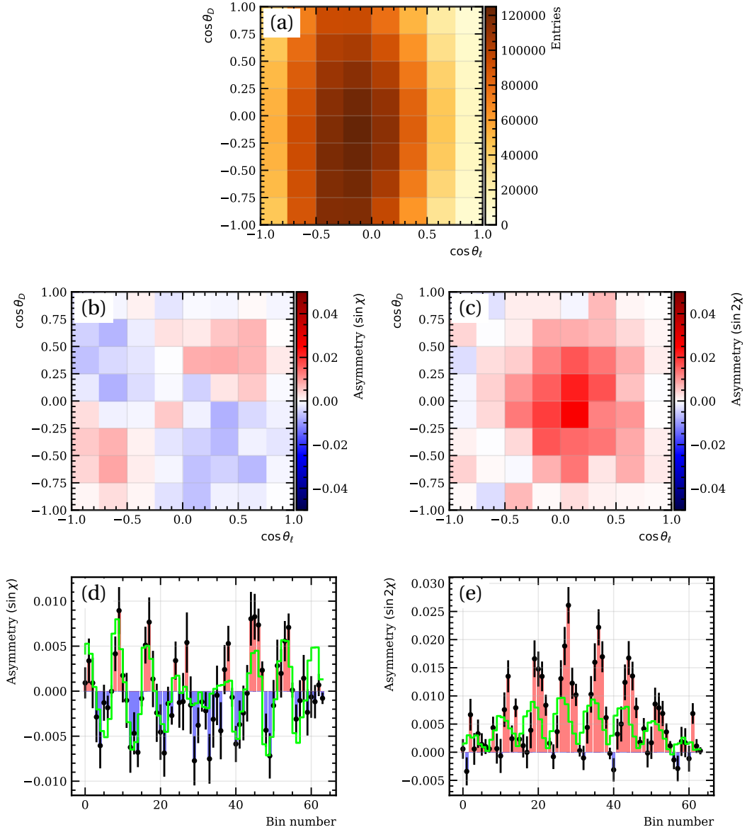
Figure 7: Binned density (a), binned 2D parity asymmetries (b,c) and flattened 1D parity asymmetries (d,e) of \sin \chi and \sin 2\chi terms in (\cos \theta_D, \cos \theta_\ell) bins integrated over q^2 for the B^+ \rightarrow D^{*0} \mu^+ \nu_\mu with \delta_D = 270^\circ . Figures (d) and (e) also show the result of the best fit in green using the RH and PT templates.
