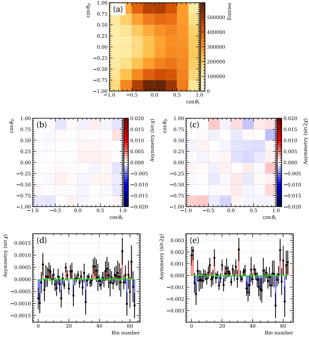
Figure 17: Binned density (a), binned 2D parity asymmetries (b,c) and flattened 1D parity asymmetries (d,e) of \sin \chi and \sin 2\chi terms in (\cos \theta_D, \cos \theta_\ell) bins integrated over q^2 for the R_z misalignment sample. Figures (d) and (e) also show the result of the best fit in green using the RH and PT templates.
