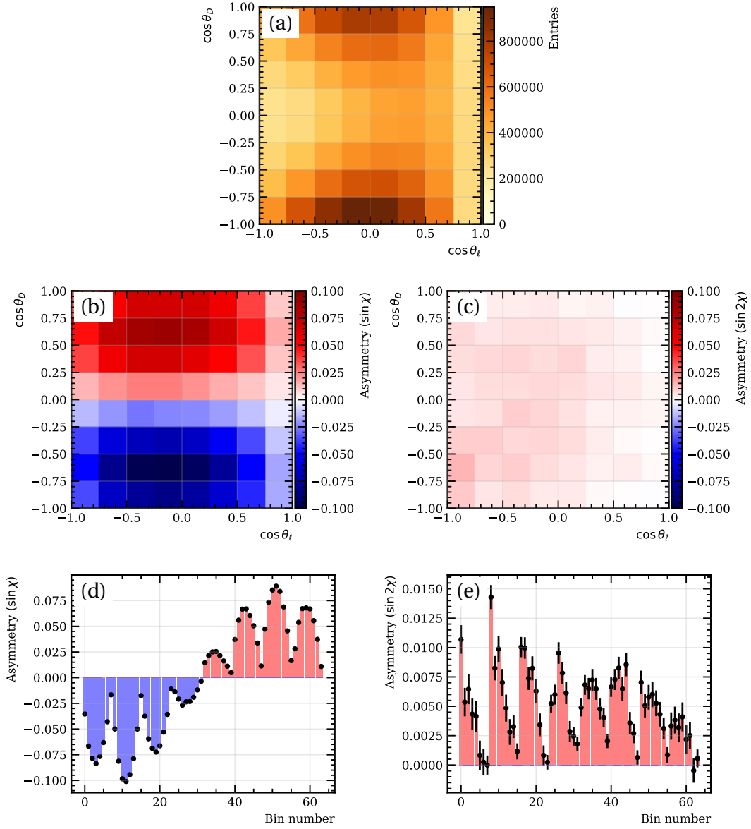
Figure 4.21: Binned density (a), binned 2D CP asymmetries (b,c) and flattened 1D CP asymmetries (d,e) of \sin\chi and \sin 2\chi terms in (\cos\theta_D, \cos\theta_\ell) bins integrated over q^2 for the B^0 \rightarrow D^{*-} \mu^+ \nu_\mu simulation sample in the NP case of \text{Im}(g_P g_T^*) = 0.1 i
