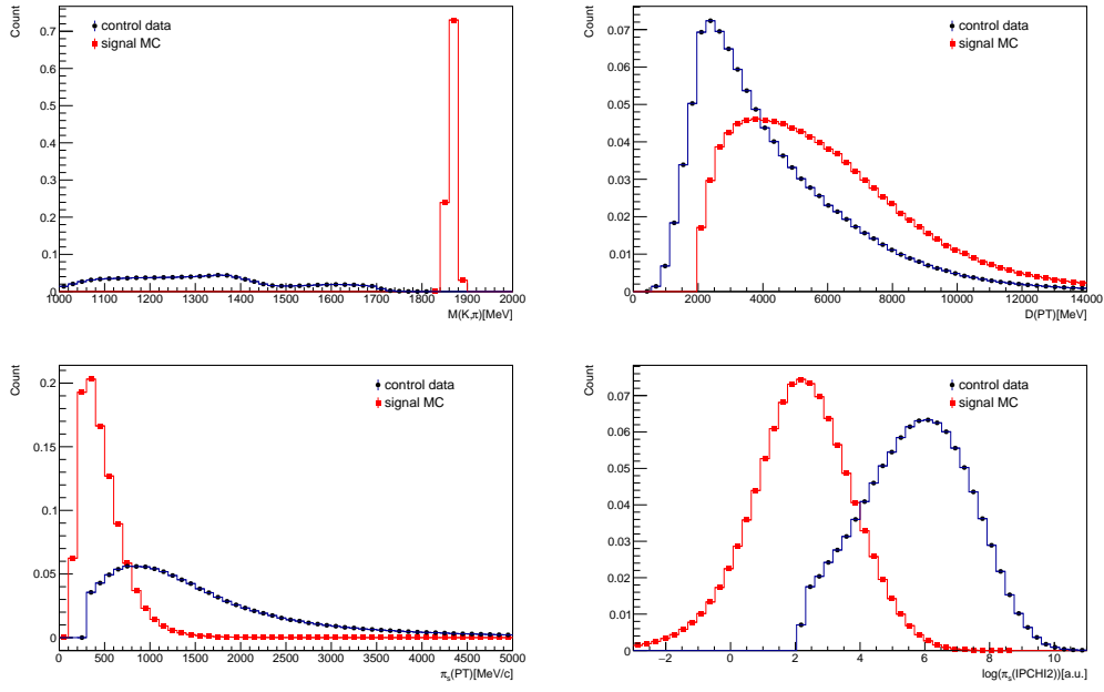
Figure 4.50: Comparison of the M(K^+\pi^-) , p_T(K^+\pi^-) , p_T(\pi_s) , \chi_{IP}^2(\pi_s) variables between the signal and control samples.
