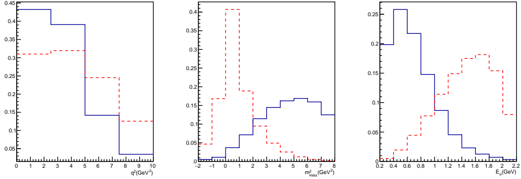
Figure 4.11: Projections of the 3D template in q^2 , m_{miss}^2 and E_\mu^* for the B^0 \rightarrow D^{*-}D_s^+ X, D_s^+ \rightarrow X\mu^+\nu_\mu sample in blue. The signal projections are shown in red for comparison.
