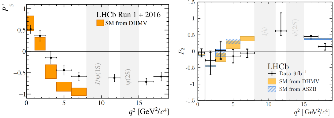
Figure 2.9: Measurements of the P_2 angular observable in B^+ \rightarrow K^{*+}\mu^+\mu^- (right) [61] and the P_5^{\prime} angular observable in B^0 \rightarrow K^{*0}\mu^+\mu^- (left) [60]. The 2.9(3)\sigma deviations from SM in the P_5^{\prime}(P_2) observables are found in the same q^2 region of 6.0 - 8.0 \text{ GeV}^2
