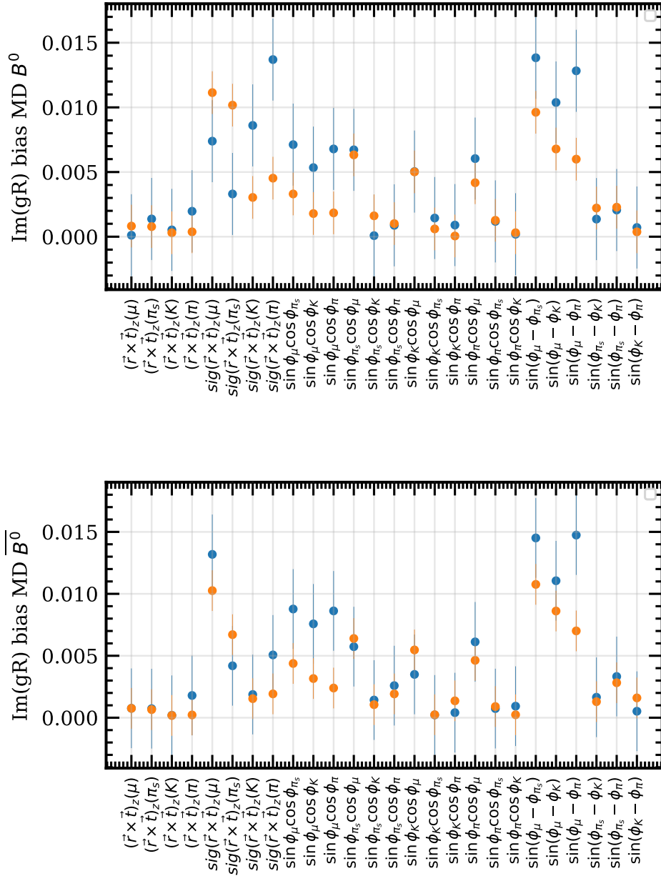
Figure 4.46: \text{Im}(g_R) biases due to all P -odd efficiency weights for signal (orange) and control (blue) samples in the MagDown B^0 (top) and \overline{B^0} (bottom) categories.
