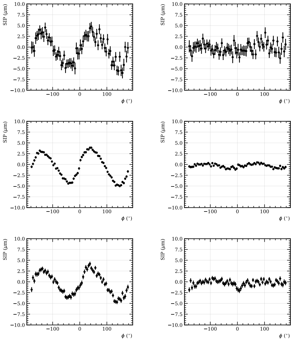
Figure 4.43: SIP vs. \phi dependence for the 2018 MagUp B^+ \rightarrow J\psi K^+ data sample for fill time < 10e3 seconds (top), fill time \in (30e3, 60e3) seconds (middle) and fill time > 80e3 seconds (bottom) before (left) and after (right) correcting for the misalignment of the VELO
