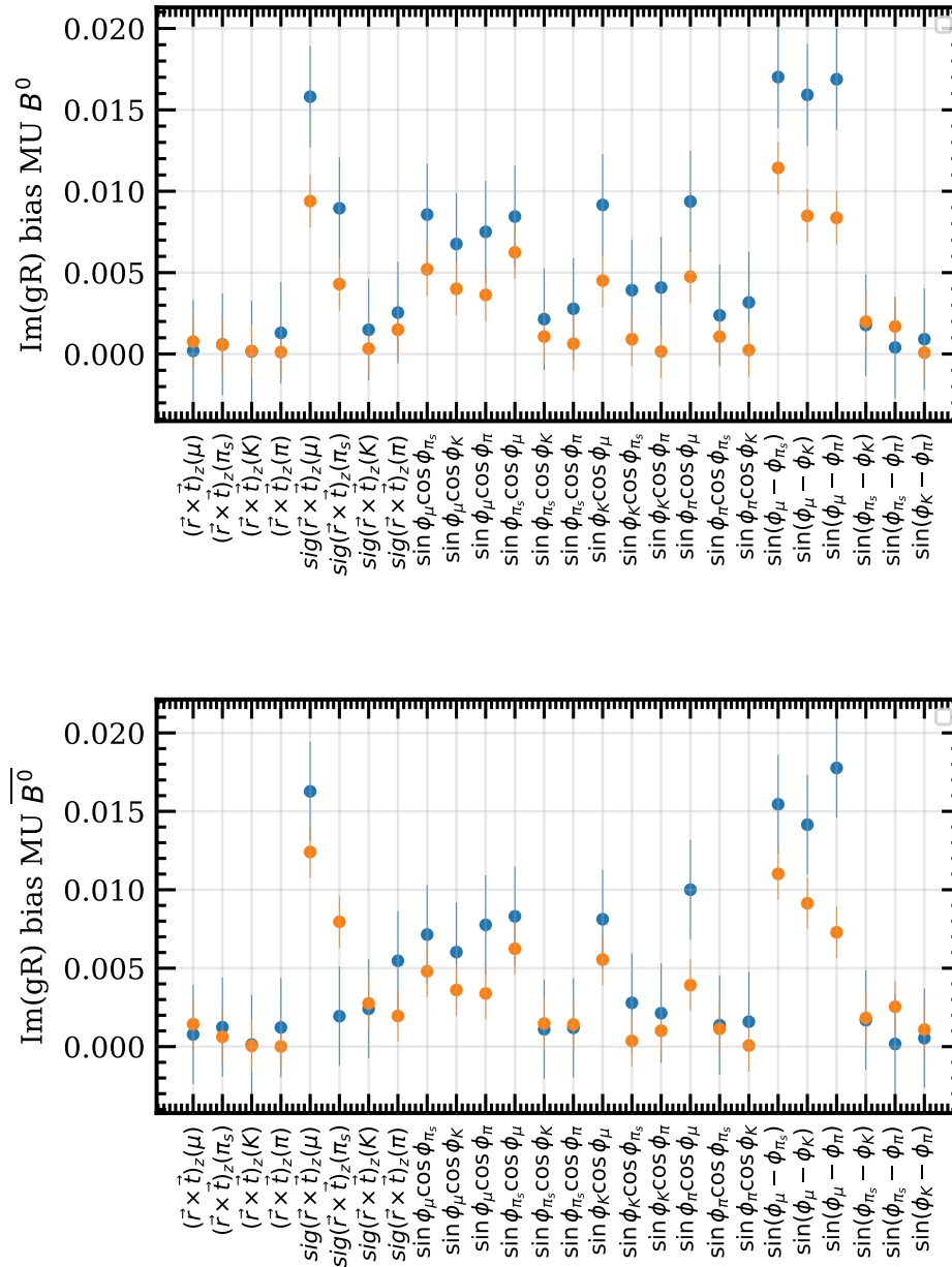
Figure 4.47: Im(g_R) biases due to all P -odd efficiency weights for signal (orange) and control (blue) samples in the MagUp B^0 (top) and \bar{B}^0 (bottom) categories.
