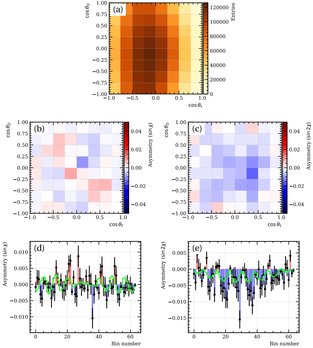
Figure 5: Binned density (a), binned 2D parity asymmetries (b,c) and flattened 1D parity asymmetries (d,e) of \sin \chi and \sin 2\chi terms in (\cos \theta_D, \cos \theta_\ell) bins integrated over q^2 for the B^+ \rightarrow D^{*0} \mu^+ \nu_\mu with \delta_D = 180^\circ . Figures (d) and (e) also show the result of the best fit in green using the RH and PT templates.
