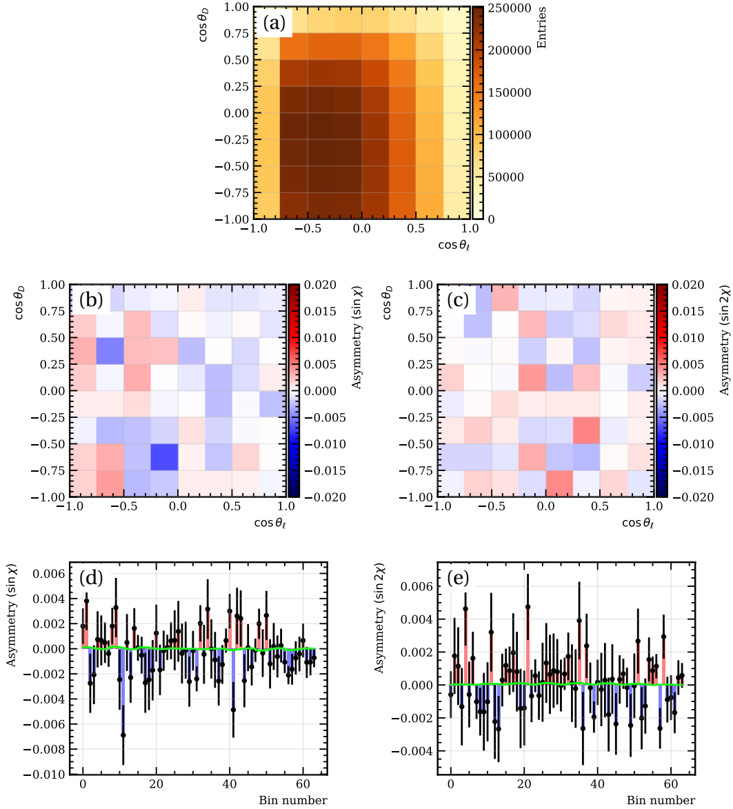
Figure 4.52: Binned density (a), binned 2D parity asymmetries (b,c) and flattened 1D parity asymmetries (d,e) of \sin\chi and \sin 2\chi terms in (\cos\theta_D, \cos\theta_\ell) bins integrated over q^2 for the B^0 \rightarrow D^- \mu^+ \nu_\mu control data sample. Figures (d) and (e) also show the result of the best fit in green using the RH and PT templates.
