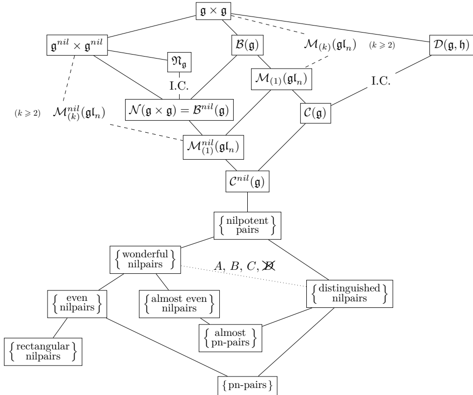
Figure 3: Doubled setting, some G -subsets/subvarieties/subschemes.
