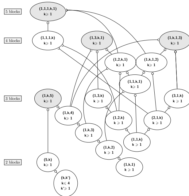
Figure 2: finite cases
