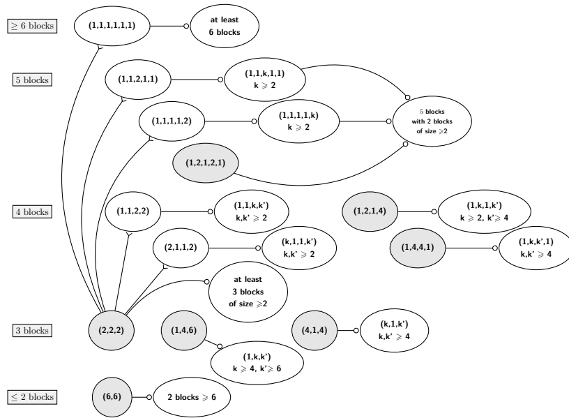
Figure 1: Infinite cases
