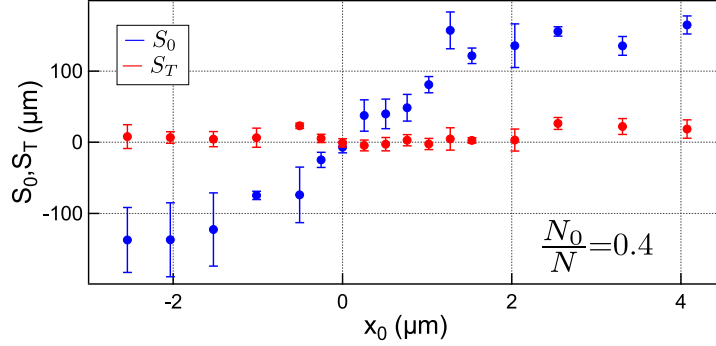
Figure 22. Measured spin displacements \{S_0, S_T\} for the thermal (red) and condensed components (blue) of the mixture as a function of x_0 for N_0/N = 0.4 for configuration (B). From such data, we extract \{\mathcal{P}_0, \mathcal{P}_T\} using a linear fit to the data in the linear region around the origin. We obtain \{\mathcal{P}_0 = 56(8), \mathcal{P}_T = -3(3)\} . Figure from [P5].
