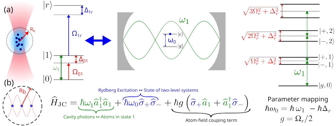
Figure 43. Mapping of either [(a) a Rydberg blocked ensemble of three-level atoms trapped in a single optical tweezer] or [(b) several individual three-level atoms in optical tweezers inside a blocked sphere] to the JC model which also describes a strongly coupled atom-cavity system. The spectrum the system is nonlinear and called the JC ladder. The dressed-states (polaritons) will be exploited to encode and process quantum information as a qudit.
