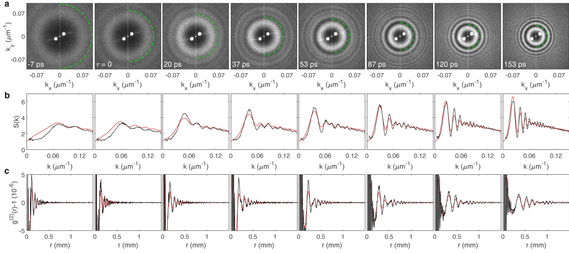
Figure 36. Analogue cosmological particle creation in a quantum fluid of light. a The static structure factor S(k_x, k_y, k_{z'} = 0) at various times after the second quench. The dashed green curves indicate the first minimum of the red curves in (b). The symmetric white points near the center of all panels are due to spurious fringes in the imaging system. b Radial profiles of (a). The black curves are the experimental data. The red curves are the prediction for analogue cosmological particle creation, from Eq. (34). c Density-density correlations. The experimental (black) and theoretical (red) curves are obtained from b by the spherical Fourier transform of Eq. (37). Figure from [P1].
