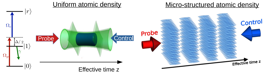
Figure 42. Overview of the experimental platform to explore strongly interacting quantum fluids of light in propagating geometry. The strong interactions between atoms excited to Rydberg states are mapped to the probe photons using Rydberg EIT. Either uniform or micro-structured atomic densities will be investigated, leading to uniform or micro-structured photon-photon interactions.
