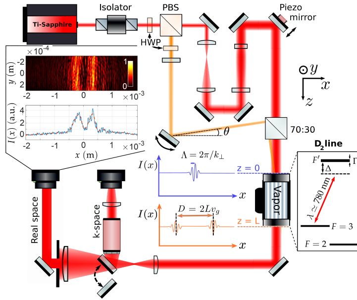
Figure 23. Experimental setup. PBS and HWP stand for Polarized Beam Splitter and Half-Wave Plate respectively. \theta is the angle between the probe (orange beam) and the optical axis defined by the pump (red beam). The probe interferes with the pump and slightly modulates its intensity. Blue inset: integrated intensity profile at the input of the medium ( z = 0 ). The wavelength \Lambda of the density modulation is given by 2\pi/k_{\perp} where k_{\perp} = k_0 \sin \theta . Orange inset: integrated intensity profile at the output of the medium ( z = L ). The distance D between the two wavepackets gives access to the group velocity of the elementary excitations in the transverse plane. The output plane is imaged on a CMOS camera. Inset on the top left: background-subtracted image obtained for \theta \approx 0 rad and associated integrated envelope profile (blue: original ; red dotted : high frequency filtered). Figure from [P4].
