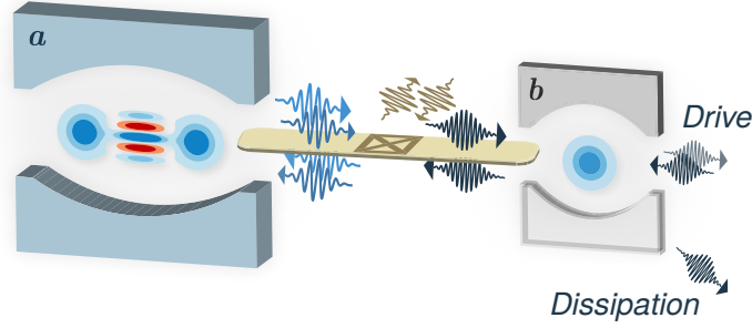
Figure 1.8: Schematic of a cat qubit mode a stabilized by a two-to-one photon exchange with buffer mode b , mediated by a nonlinear circuit element (middle) and a pump at the appropriate differential frequency. The buffer mode is driven and dissipates photons to the environment.
