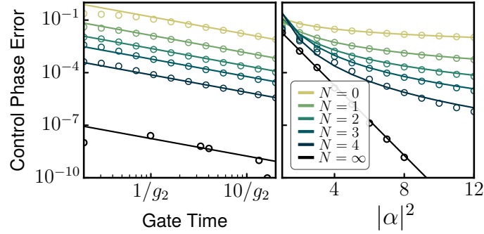
Figure 3.10: Gate-induced control phase errors for a CNOT gate with a locally flat drive Hamiltonian as in (3.26). Left: fixed cat size, |\alpha|^2 = 8 . Right: fixed gate time T = 10/g_2 . Dissipative stabilization is acting on the control qubit only, with \kappa_b = 8g_2 . Lines show numerical fits of the form p_{Z_C} \propto T^{-1}|\alpha|^{-2N} (color) and p_{Z_C} \propto T^{-1} \exp(-2|\alpha|^2) (black). Markers show numerical data.
