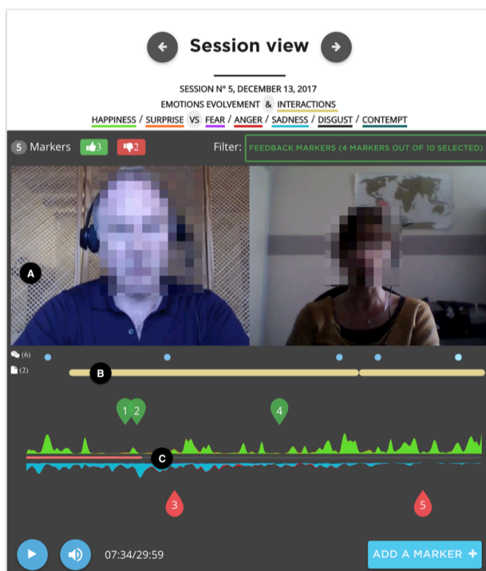
Figure 4.11: Session View.
