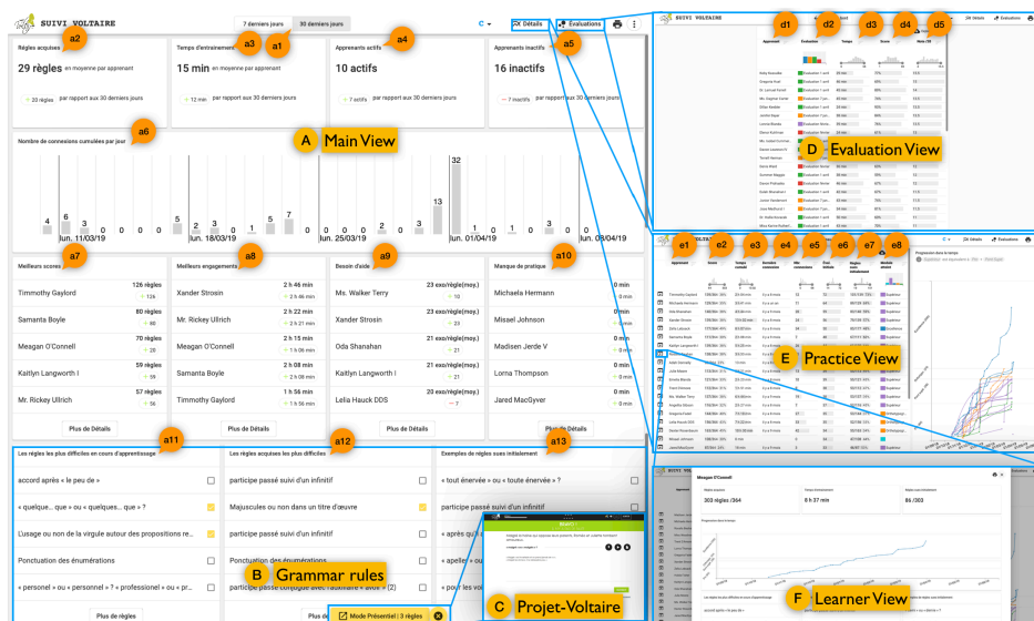
Figure 5.6: PROGDASH User Interface.
