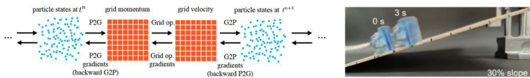
Figure 2.3: Illustration of the Material Point Method for simulating soft robots: particle-to-grid scheme and grid-to-particle transfers implemented in the ChainQueen simulator [Spi+23] (left), and an example of a locomoting soft robot with a MPM-based controller [Kob+23] (right).
