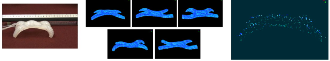
Figure 2.11: Example of MOR for a multigait soft robot (left) actuated by 5 pneumatic actuators from [GD18]. The 5 first basis vectors (middle) and the reduced integration domain (right) are displayed. A given state of the multigait is approximated by a weighted sum of the basis vectors.
