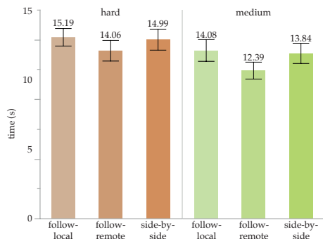
Figure 5. TCT in seconds for each VIDEO × LAYOUT condition. Bars show the 95% confidence intervals.
