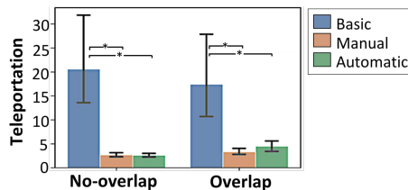
Figure 12: Mean Teleportations by TECHNIQUE \times LAYOUT. Error bars show 95% CI.
