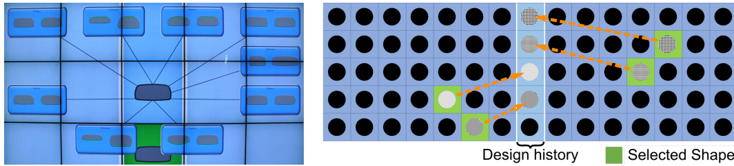
Figure 3.4: Updated version of ShapeCompare : (left) the selection widget shows small thumbnails with minimum and maximum shape modifications for all parameters and (right) all selected shapes are displayed in the middle of the next row to improve the visibility of the design history.
