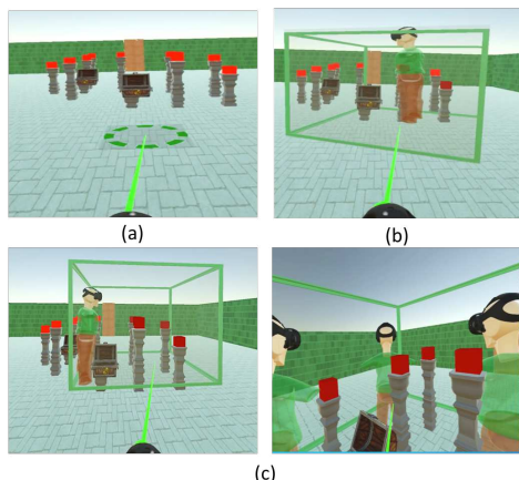
Figure 9: Three conditions for TECHNIQUE: (a) Basic teleportation; (b) Manual technique selected from EXPERIMENT 1; (c) Automatic technique: the user selects their future virtual workspace among relevant options (left), or selecting avatars in overlapping conditions (right).
