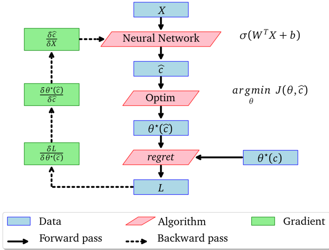
Figure 2.16 – In Decision-Focused Learning , the regret is taken into account during the training of the Neural Network that forecasts \hat{c} . The chain rule is applied as usual and the gradient of the solution to the optimization problem with respect to its input \frac{\partial \theta^*(\hat{c})}{\partial \hat{c}} has to be estimated.
