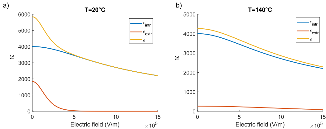
FIGURE 1.13: Dielectric permittivity as a function of the electric field for different temperature for \text{KNa}_{0.5}\text{Nb}_{0.5}\text{O}_3 - \text{SrTiO}_3 ceramics [Liu+16]; (a) T=20^\circ\text{C} ; (b) T=140^\circ\text{C}
