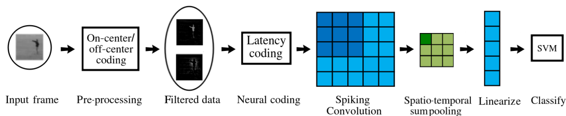
Figure 4.1: General recognition pipeline that serves as a basis in the subsequent contribution chapters.
