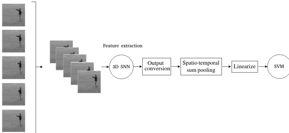
Figure 6.5: Introducing an input video for spatio-temporal feature extraction using a 3D architecture.
