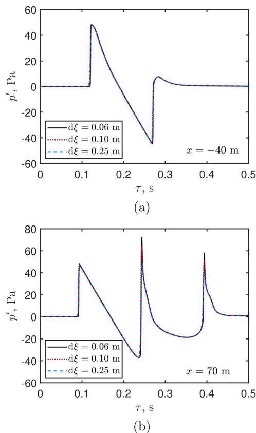
FIG. 17. (Color online) Terrain depression, N-wave—time signals obtained using different mesh sizes at positions (a) x = -40 m and (b) x = 70 m along the terrain depression ground profile.
