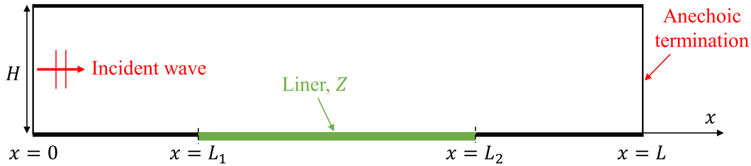
Fig. 20. Schematic of the 2D lined duct.
