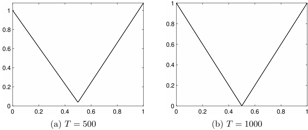
Figure 4.6: Convergence factor w.r.t. \theta
