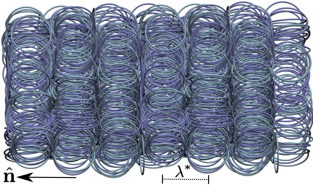
FIGURE 4.1. Representative configuration of the smectic-A (SmA) phase formed by a system of N = 500 rigid rings obtained by molecular dynamics simulations. This system is modelled as a collection of n_b = 56 tangent beads of diameter \sigma interacting via a soft WCA potential. The radius of the rings (from the centre of the particles to the centre of the peripheral beads) is r = 8.92\sigma . The particle density is \rho r^3 = Nr^3/V = 1.5 which corresponds to a very low packing fraction \phi = \pi N n_b \sigma^3 / (6V) = 0.062 . The system has been replicated along the direction of the layers to aid the visualisation of the SmA phase. The typical lamellar spacing is indicated by \lambda^* . The rings are aligned anti-nematically with their normals pointing perpendicular to the lamellar director \hat{\mathbf{n}} . Traces of inter-layer rings with transverse, nematic order are visible in the centre of the image.
