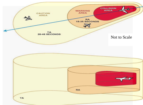
Figure 5.10: TCAS protected volume
