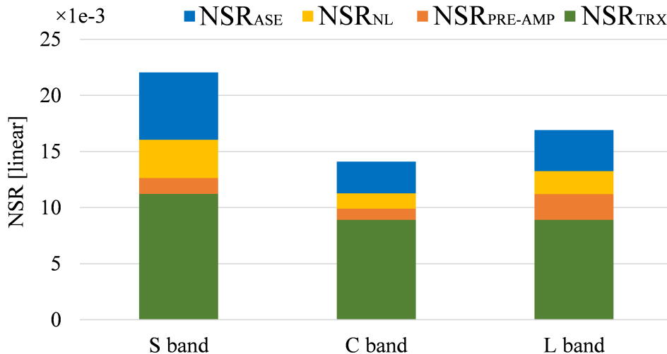
Fig. 4.7: Contributions per band, NSR TRX (green), NSR PRE-AMP (orange), NSR NL (yellow) and NSR ASE (blue) from bottom to top.
