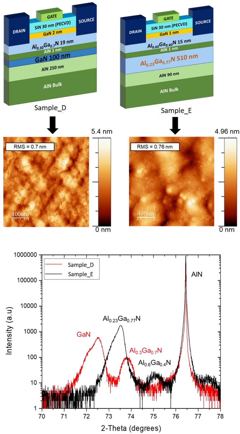
Fig. 3. 9 Cross-sectional schematics of GaN channel (Sample_D) and AlGaN channel (Sample_E) heterostructures on bulk AlN along with their AFM scans and XRD scans
