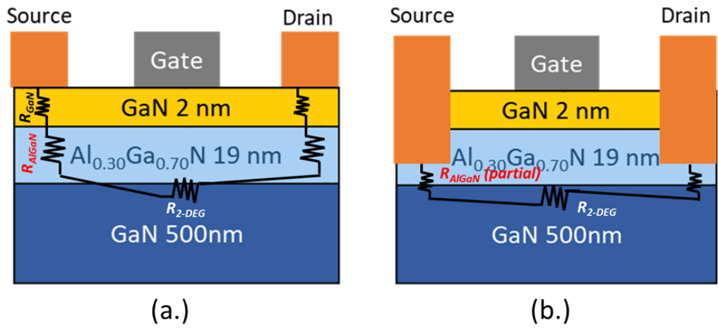
Fig. 1. 6 Schematic of AlGaN/GaN HEMTs source/drain contacts with (a.) contacts deposited on top of barrier and (b.) barrier etched contacts along with their contact resistances.
