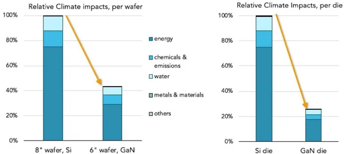
Fig. 1.23 Comparison of Fab energy/material usage for GaN and Si (source: www.powerelectronicsnews.com )
