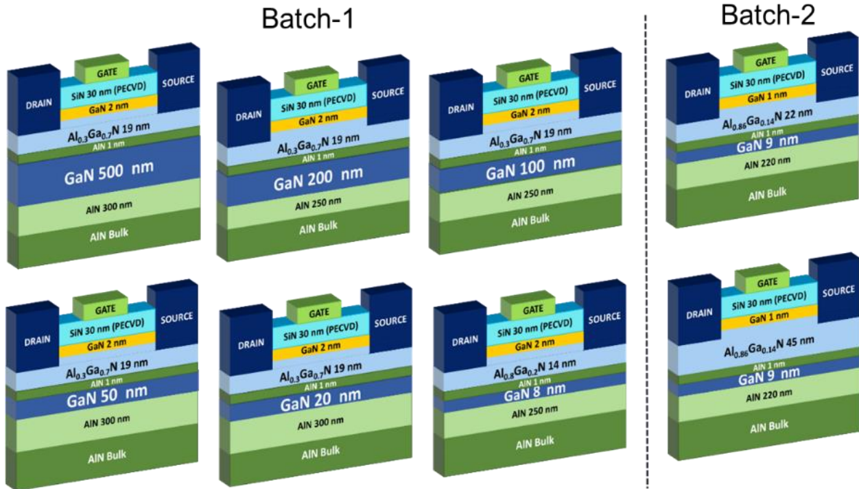
Fig. 2.2 Cross-sectional schematic structures of fabricated GaN channel MISHEMTs on AlN
