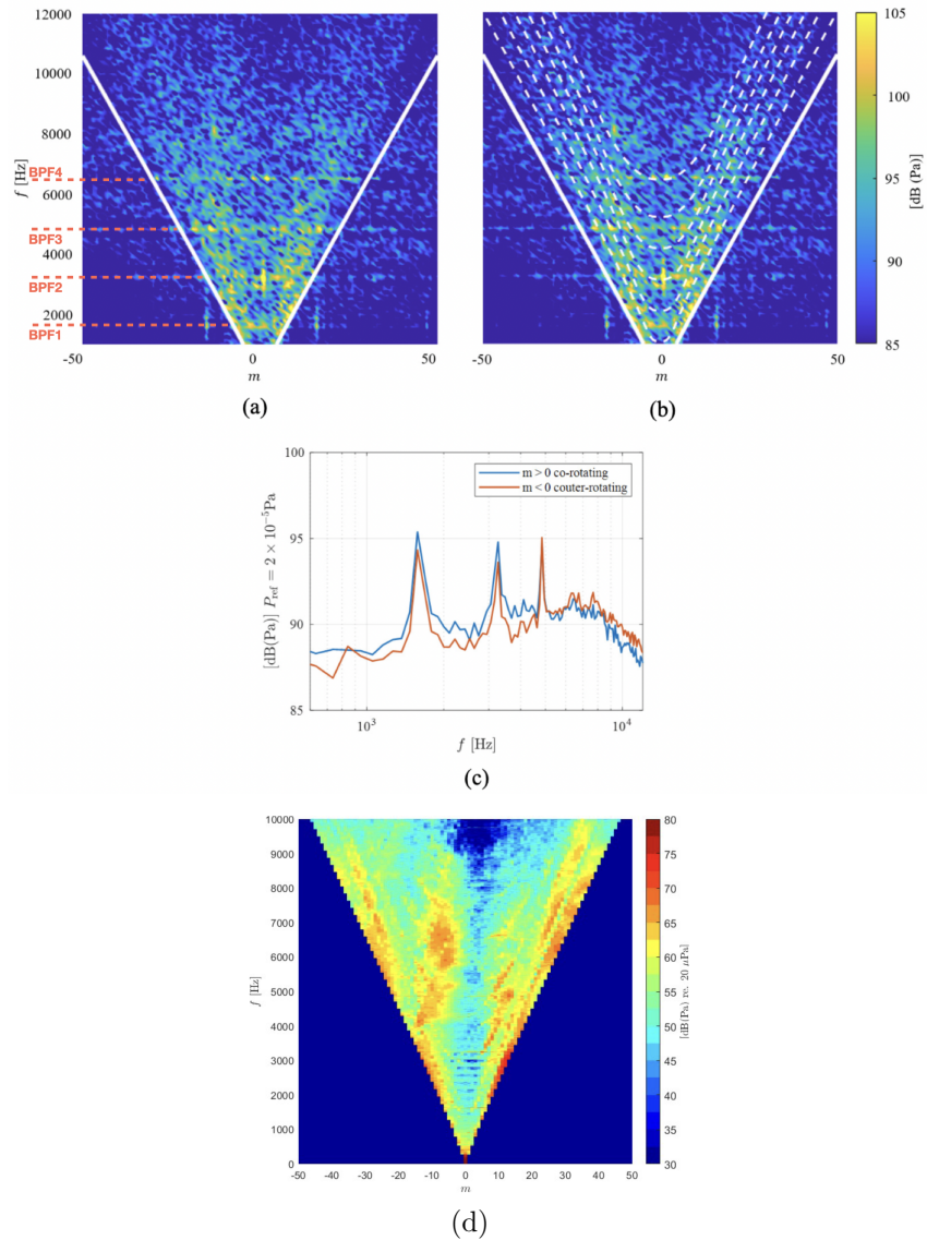
Figure 5.32: Azimuthal mode detection plots at the exhaust section. (a,b) 360° LES: The frequency is plotted against the azimuthal mode order m , and the modes are colored by their amplitude. (c) Integrated mode spectra over co-rotating ( m > 0 ) and counter-rotating ( m < 0 ) modes, (d) Experiment: The frequency is plotted against the azimuthal mode order m (from [11])
