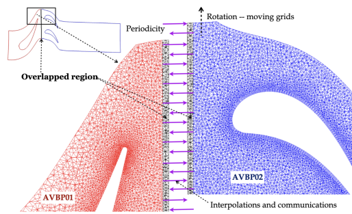
Figure 3.3: Communications framework of coupling rotor/stator interface. (from [2])
