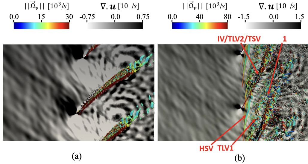
Figure 5.23: Instantaneous contours of dilatation rate and iso-surfaces of Q-criterion ( Qc_r^2/U_0^2 = 100 ) colored by the vorticity magnitude, around the rotor blades, at two spanwise positions, (a) 80% and (b) 98%. (from [13])
