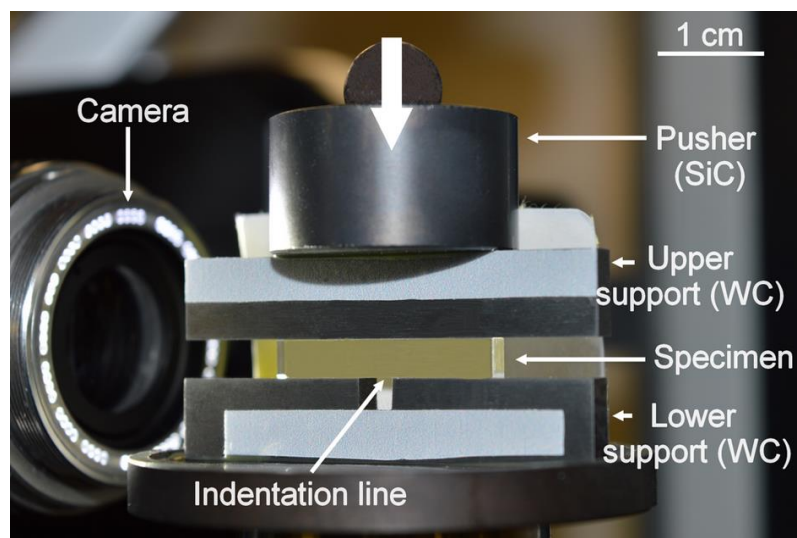
Fig. III.5: Compression fixture with indented specimen (Planilux).
