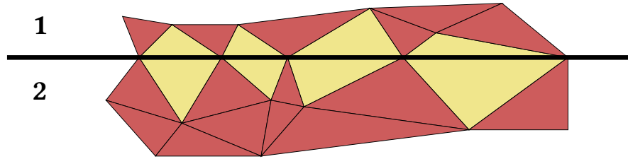
Figure 28: In this figure the computation domain is partitioned into two subdomains, sharing the thick black line as interface. The triangles which share an edge with the interface are called border cells and are painted in yellow. The other triangles are called interior cells and are painted in red.
