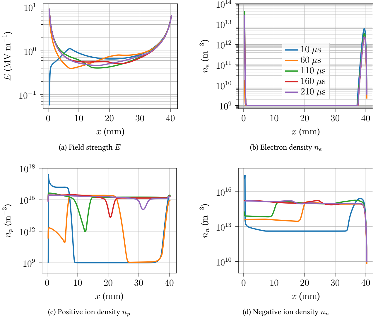
Figure 5.2: Evolution of the field strength and specie densities of the 400 SGCC-2 simulation
