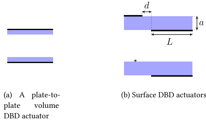
Figure 1.17: Illustration of some DBD actuators. Electrodes are colored in black, dielectric barriers in blue.
