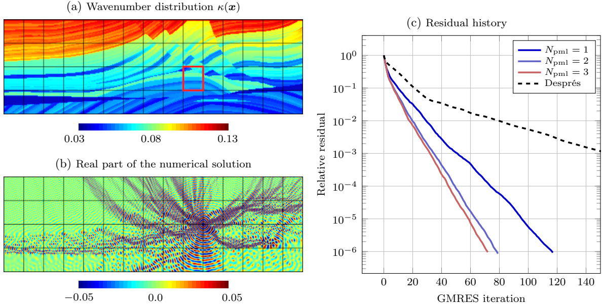
Figure 3.12: Marmousi benchmark: (a) wavenumber distribution, (b) numerical solution and (c) residual history. Parameters: frequency f = 30\text{Hz} , rectangular finite elements with first-degree polynomial basis functions, characteristic mesh size h \approx 10\text{ m} . Adapted from [A15].
