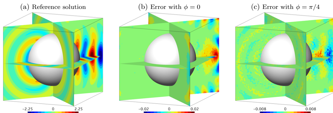
Figure 2.3: Cuboidal truncated domain: real part of the reference solution (a) and simulation error with a Padé-type HABC ( N = 2 and either \phi = 0 (b) or \phi = \pi/4 (c)) and the corner/edge compatibility relations. Parameters: domain \Omega = [-1.41, 1.41]^3 , sphere of radius R = 1 , plane wave u^{\text{inc}}(\mathbf{x}) = e^{i\kappa x} , boundary condition on the disk \partial_n u = -\partial_n u^{\text{inc}} , wavenumber \kappa = 10 , second-order curvilinear triangular elements, second-degree polynomial basis functions, mesh density n_\lambda \approx 10 . Reproduced from [A9].
