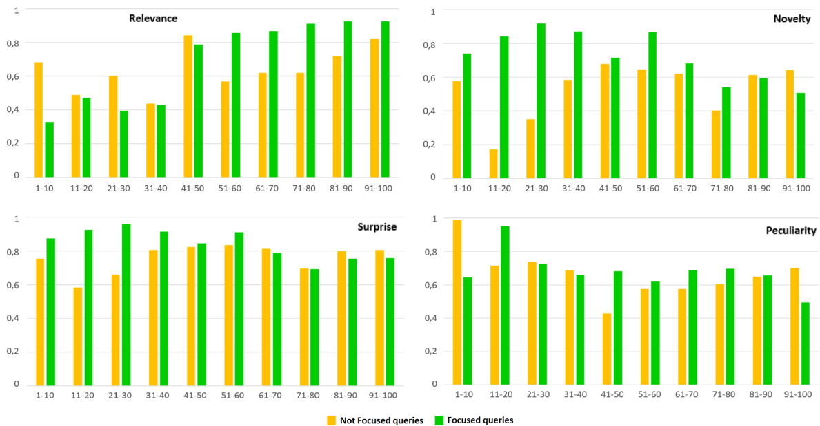
Figure 3.2: Evolution of the four interestingness measures (y-axis) with respect to the % progress in a exploration (x-axis) for focused vs non-focused queries
