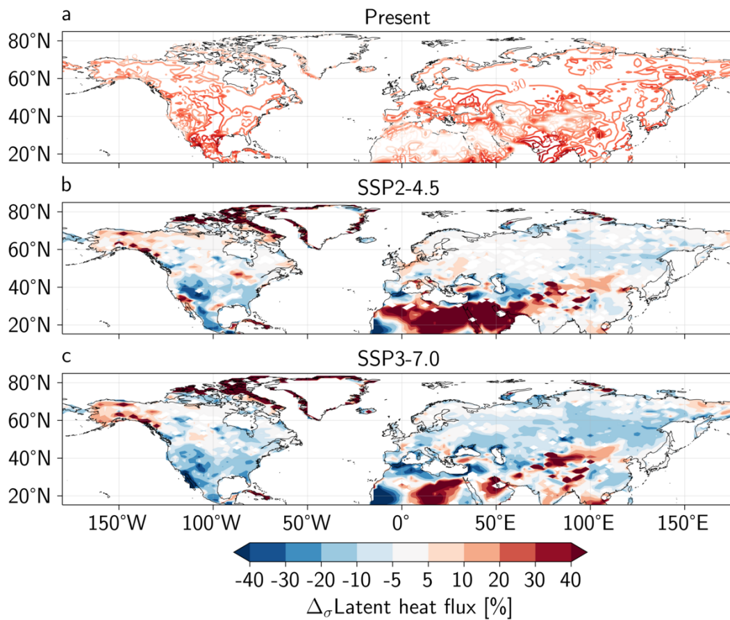
Figure A.24: Standard deviation of the summer distribution of daily latent heat flux in (a) the present simulation (°C, contours) and standard deviation anomaly in (b) SSP2-4.5 and (c) SSP3-7.0 (%). For panels b and c, the anomalies are computed with respect to the present simulations. The grid point where the normalized anomaly with respect to the present simulation is below 5% in absolute value are colored in white.
