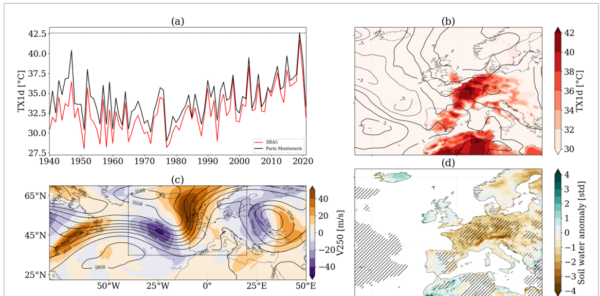
Figure 1. (a) Annual maximum temperature for the Paris Montsouris station (black) and the grid point where the station is located for ERA5 (red). The black dashed line corresponds to the temperature reached on the 25 July 2019 at the Paris Montsouris station. (b) Daily maximum 2 m air temperature (colors) and daily mean 500 hPa temperature anomalies (contours). (c) Daily mean meridional wind at 250 hPa (colors) and geopotential height at 500 hPa (contours). (d) Daily mean normalized soil moisture anomaly (colors) and hourly mean 2 m specific humidity at the time when maximum 2 m air temperature is reached (hashed). The hashed regions represent anomalies below -0.5 standard deviation. All maps are drawn for the 25 July 2019.
