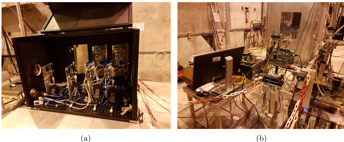
Figure 5.10.: 5.10a : The box with planes 1 and 2 of TDCPix, close together. Picture taken during the test beam in 2017. 5.10b : The TimePix3 telescope (gray box) and plane 3 of TDCPix ("L" structure in front of it). Picture taken during the test beam in 2017.
