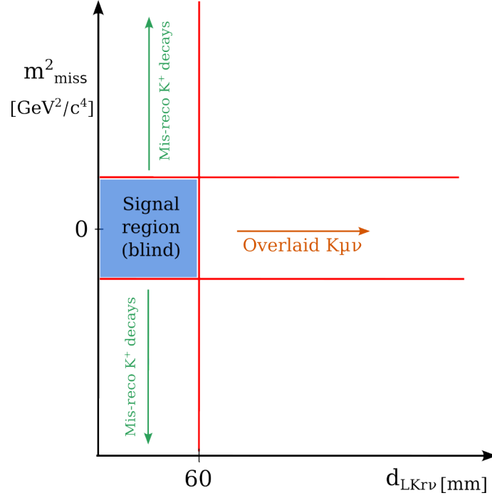
Figure 4.3.: Schematic 2D representation of the signal region, identified by the two variables d_{\text{LKr}\nu} and m_{\text{miss}}^2 .
