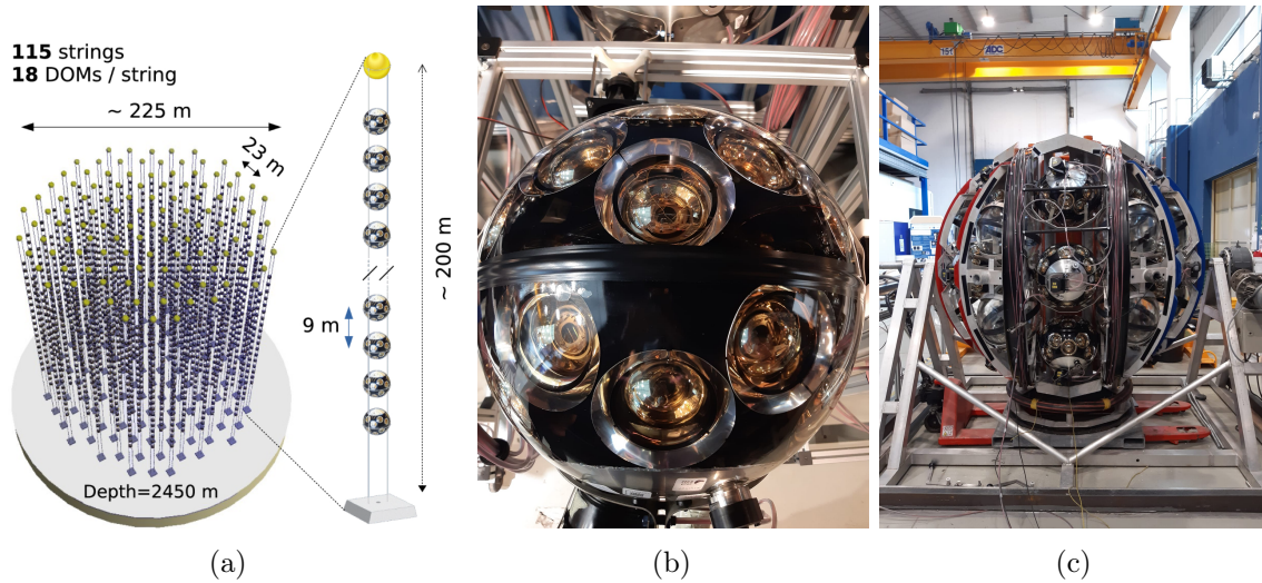
Figure 1.10.: 1.10a : Schematic of the layout of the completed KM3NeT/ORCA site, from [16] . 1.10b : a DOM being calibrated, photo taken in the CPPM assembly lab. 1.10c : photo of a launch vehicle deployment that exploits the unfurling of the string, taken in the CPPM assembly lab.
