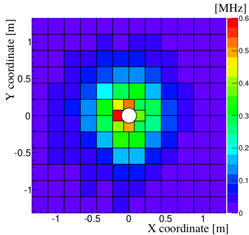
Figure 3.15.: MUV3 illumination from [81].
