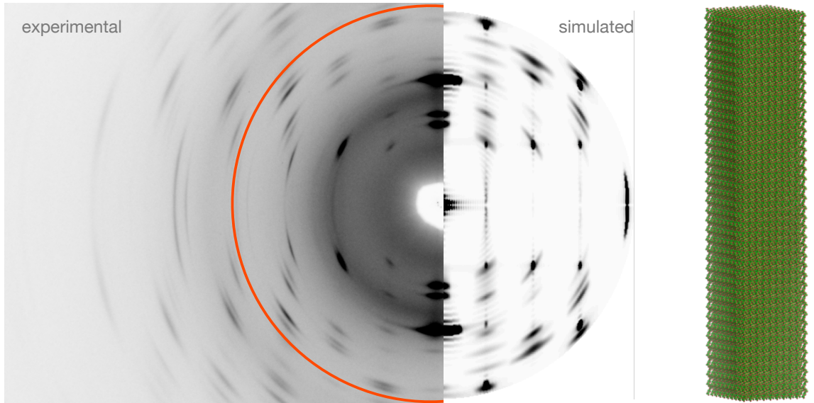
Figure 30: Experimental versus calculated scattering profiles for a cylindrically-averaged intensities of a fibril crystal.
