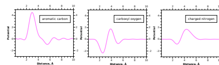
Figure 46: Knowledge-based solvation scoring functions between the oxygen of a water molecule and protein atoms as a function of the separation distance. Left: water – aromatic carbon. Middle: water – carboxyl oxygen (like in aspartic and glutamic acids). Right: water – charged nitrogen (like in lysins). Was developed for [137].
