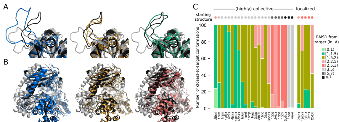
Figure 25: Examples of predictions and random sampling assessment. A-B. Superimposition of the predicted conformations (in color) onto the known starting (in grey) and target (in black) structures. The conformations in blue were produced by classical NMA while those in other colors were produced by NOLB. The amplitude of the modes were either determined using the knowledge of the target state (on the left and in the middle) or randomly sampled (on the right, with colors matching panel C). A. Transition of actin upon binding to DNase I (1atn:r). The initial RMSD is 2.7 Å and the motion involves 10% of the protein atoms. B. Closing of the diaminopimelate dehydrogenase (3dap-1dap). The initial RMSD is 4.2 Å and the motion involves about half of the protein atoms. C. RMSDs computed between the 100 closest-to-target randomly sampled conformations and the target structure. In total, 10 000 conformations were generated for each protein. The proteins are split into two groups, depending on the type of transition. Within each group, they are ordered according to the RMSD between the starting and target structures, indicated by the colored dots. The x -axis lists the PDB codes.
