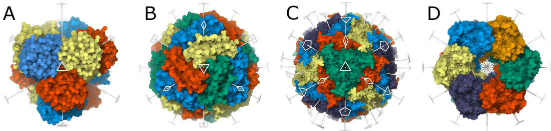
Figure 11: Four examples of symmetric assemblies with their axes. All of these are seen from a 3-fold axis except for the last one, seen from a 6 fold axis. The order n of each axis is represented with a regular n -gone, except of order 2 represented with a rhombus. A: A tetrahedral assembly (1doi) with the RMSD loss of 0.36 Å. B: An octahedral assembly (1bfr) with the RMSD loss of 0.22 Å. C: A perfect icosahedral assembly (1stm) with the RMSD loss of 0.0 Å. D: A dihedral D_6 assembly (1f52) with the RMSD loss of 0.20 Å.
