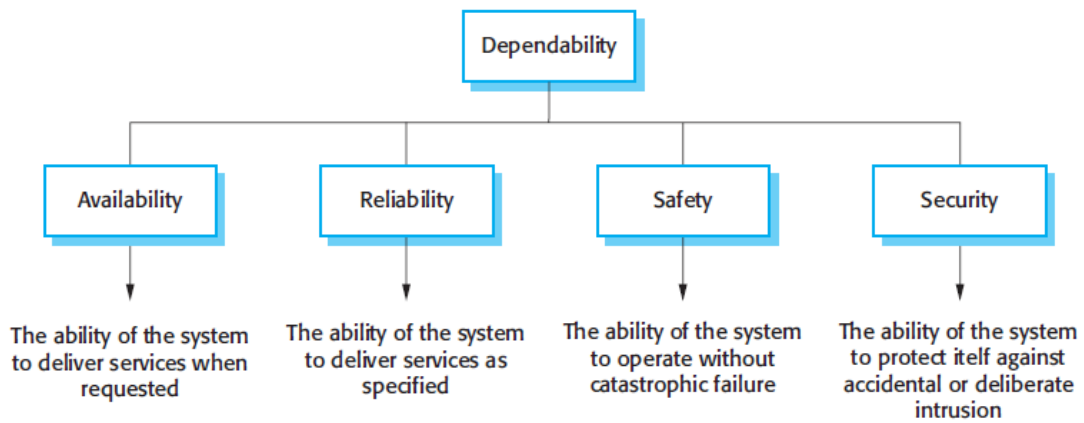
FIGURE 1.9 – Sous-taxonomie NFR - dependability [Som11]
