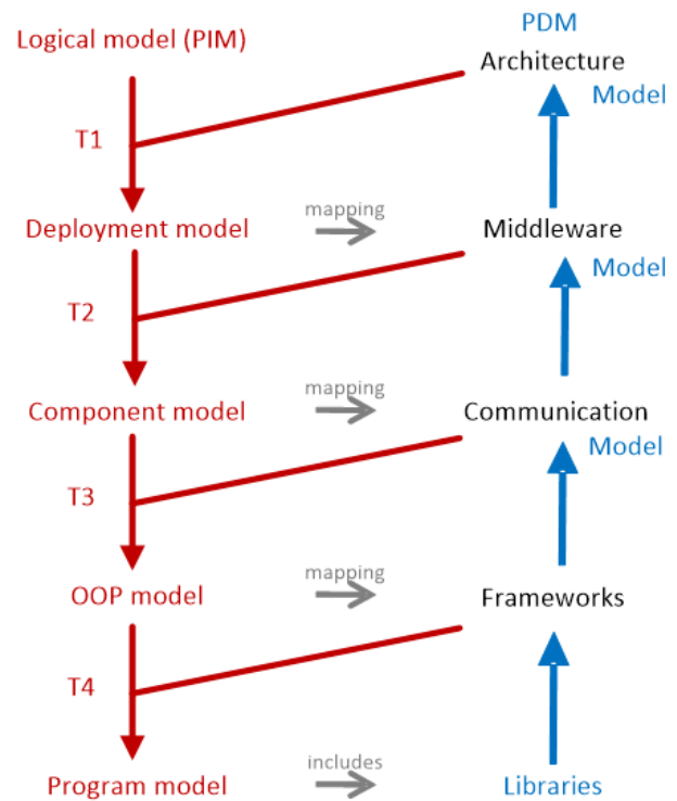
FIGURE 4.9 – Macro-transformation process
