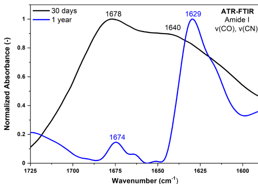
Figure 11 Exemplary, normalized ATR-FTIR spectrum of TKPAES in the Amide I ( 1700\text{-}1600\text{ cm}^{-1} ) region. Peptide dissolved in NaOH+PBS after 30 days of incubation at 37^{\circ}\text{C} and one year. C_{\text{pep}} = 500\text{ }\mu\text{M} .
