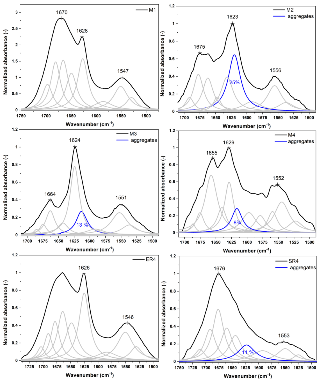
Figure 60 Normalized ATR-FTIR spectra of air-dried films of mutants and R4 fragments with sub-bands obtained from the curve fitting procedure in the amide bands region ( 1750\text{-}1490\text{ cm}^{-1} ).
