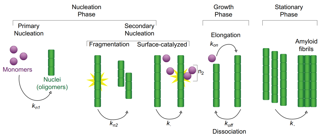
Figure 3 Schematic representation of the aggregation mechanism, where k_{n1} , k_{n2} , k_+ , k_{on} , k_{off} , k_+ represent rate constants. Adapted from [9], [24].
