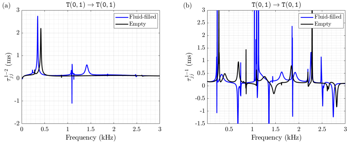
Figure 4.18: Time of flight in: (a) transmission and (b) reflection for the joint considering the mode T(0, 1) . Results for fluid-filled and empty pipes are plotted in blue and black lines, respectively.
