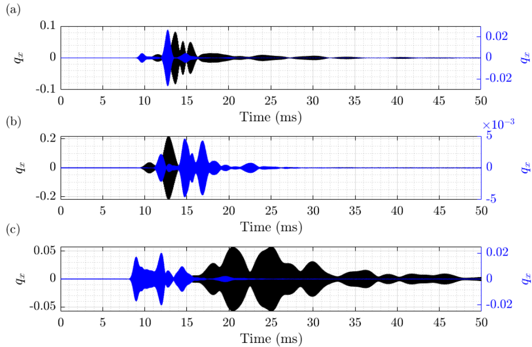
Figure 3.14: Measured time signals for an input flexural wave packet at 16.1 kHz (black) and 27.3 kHz (blue): (a) reflected flexural wave packet, (b) reflected longitudinal wave packet and (c) reflected shearing wave packet.
