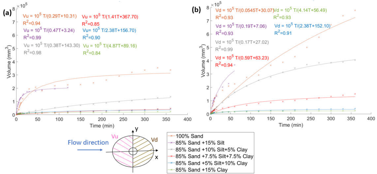
Figure IV.17: Temporal evolution of the scour volume (a): for the upstream part ( V_u ), (b): for the downstream part ( V_d ), the scheme illustrates the corresponding value of the volume for the upstream part V_u , and for the downstream part V_d
