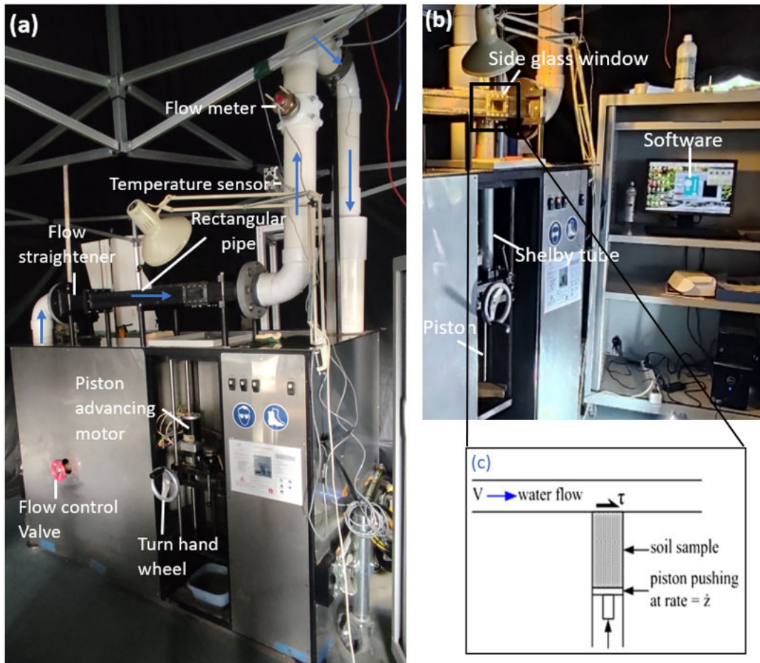
Figure II.23: Erodimer Erosion Function Apparatus (EFA), (a): overview, (b): test section, (c): conceptual diagram of soil erosion sample [50], the direction of the flow is indicated by blue arrows
