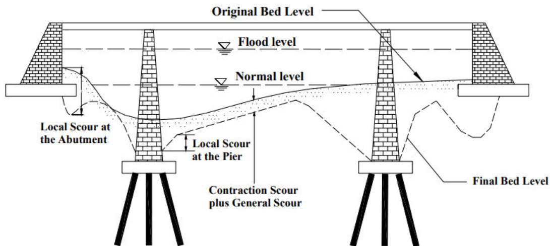
Figure I.1: Sketch of the various types of scour in a bridge cross-section; Wang 2004 [250]
