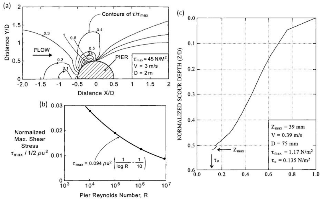
Figure I.32: Maximum shear stress around cylindrical pier \tau_{max}(\text{pier}) ; Briaud et al. 1999 [56] (data from Wei et al. 1997 [252]) (a) Contour plot showing the distribution of shear stress; (b) Relationship between the maximum shear stress and Reynolds Number; (c) variation in shear stress at the scour hole's bottom function of its depth
