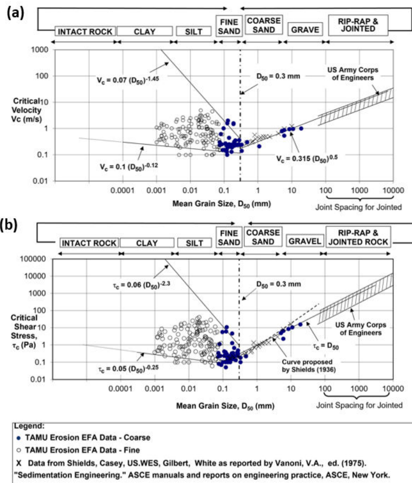
Figure I.13: Correlation between mean particle size D_{50} and (a) : the critical velocity v_{cr} , (b) : the critical shear stress \tau_{cr} ; Shaffi et al. 2023 [218]
