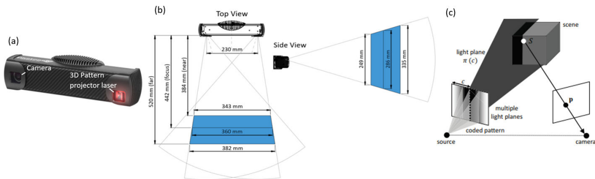
Figure II.17: PhoXi 3D Scanner S, (a): main components, (b): Scanning volume, (c): Structural light 3D imaging principle [112]
