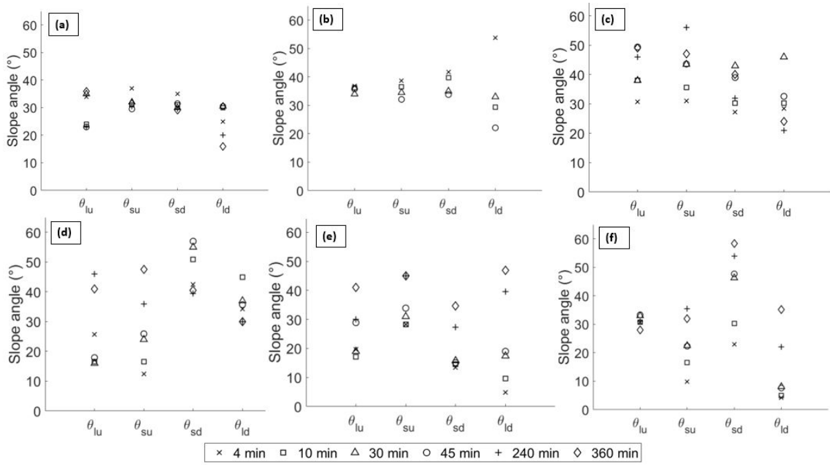
Figure IV.11: Slope angles within the scour hole; (a): 100% sand, (b): M1 mixture (85% sand+15% silt), (c): M2 mixture (85% sand +10% silt +5% clay), (d): M3 mixture (85% sand +7.5% silt +7.5% clay), (e): M4 mixture (85% sand +5% silt +10% clay) and (f): M5 mixture (85% sand +15% clay); \theta_{lu} , \theta_{su} , \theta_{ld} , \theta_{sd} are the longitudinal slope upstream, average side slope upstream, longitudinal slope downstream and average side slope downstream respectively
