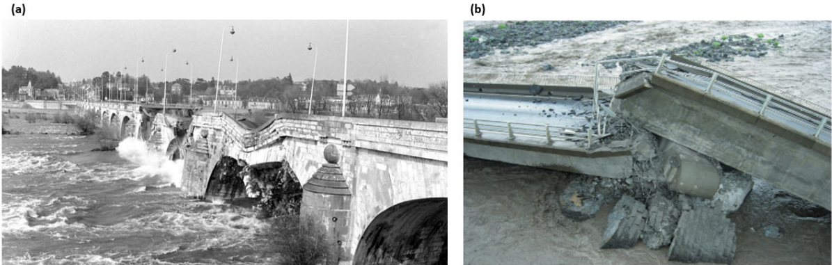
Figure 1: Examples of French bridge collapse due to scour : (a): Wilson bridge in Tours (1978) [195], (b): the bridge over the Saint-Étienne river on Reunion Island (2007) [62]
