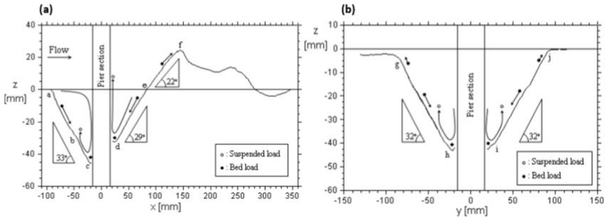
Figure I.15: Scour hole profile in cohesionless bed (a): longitudinal section; (b): transversal section; Umeda et al. 2008 [244]
