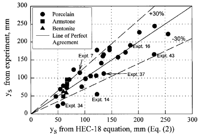
Figure I.21: Comparison between extrapolated equilibrium scour depth and the HEC-18 prediction in clay; Ting et al. 2001 [241]
