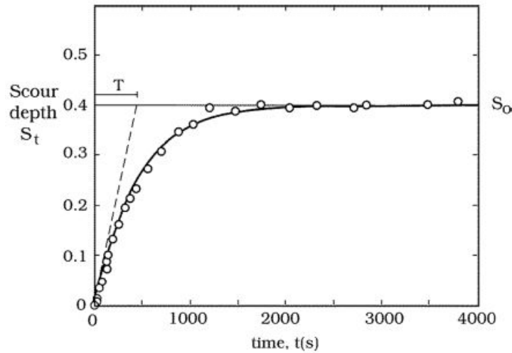
Figure I.18: Exponential law for scour depth over time with determination of the time scale; Petersen et al., 2012 [194]
