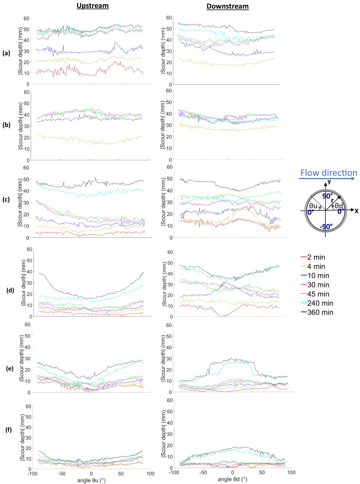
Figure IV.6: Scour depth as a function of azimuth angle upstream ( \theta_u ) and downstream ( \theta_d ) for points at radial coordinate r between 17 mm and 19 mm, (a): 100% sand, (b): 85% sand+15% silt, (c): 85% sand +10% silt +5% clay, (d): 85% sand +7.5% silt +7.5% clay, (e): 85% sand +5% silt +10% clay and (f): 85% sand +15% clay, the scheme illustrates the corresponding value of the azimuth angle for the upstream and the downstream part
