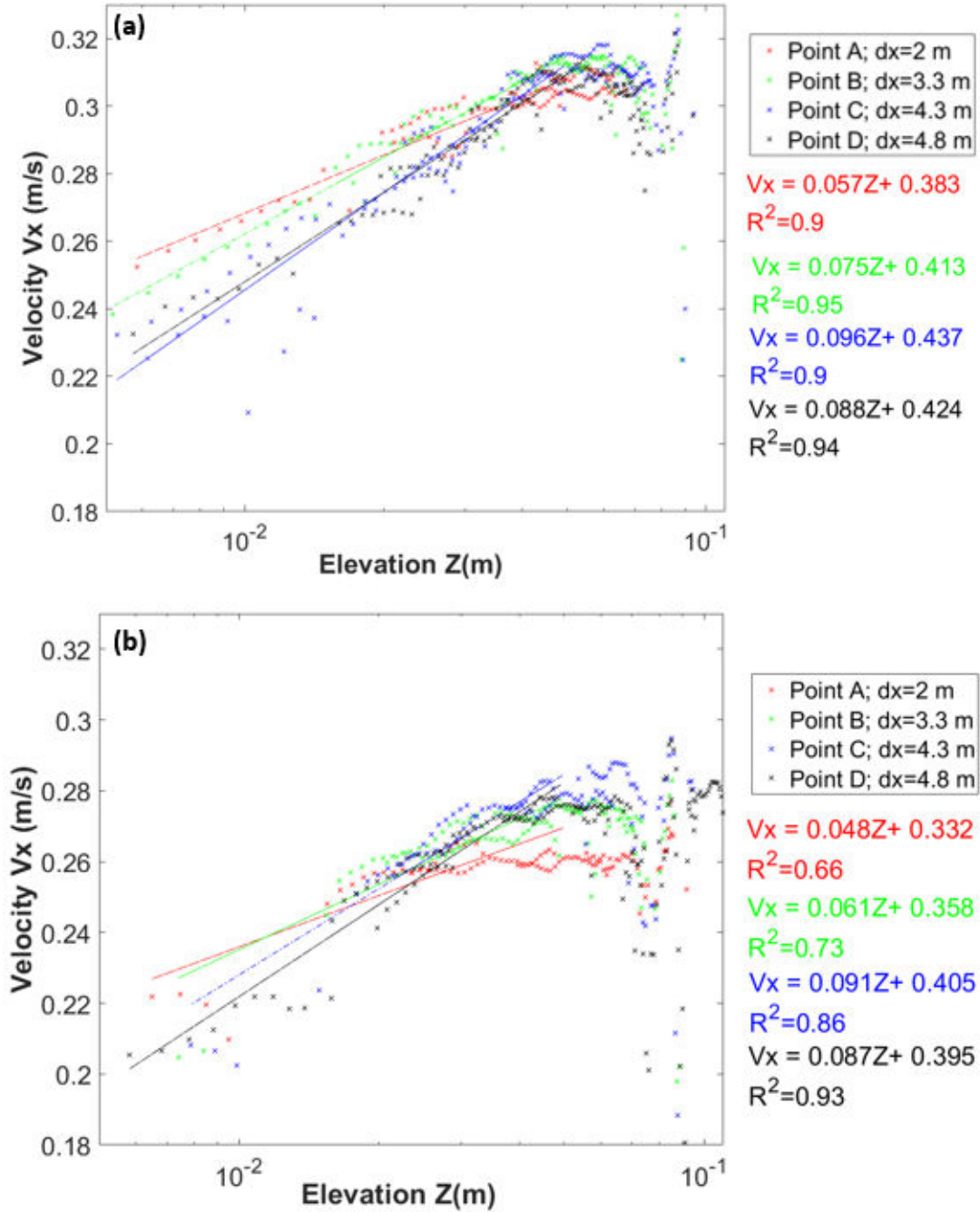
Figure II.14: Evolution of the mean velocity profiles in the longitudinal axis of the flume as a function of the axial distance with respect to the initial slope of the false bottom (dx), (a) : hydraulic condition 1 (with medium sand) (b) : hydraulic condition 2 (with fine soils)
