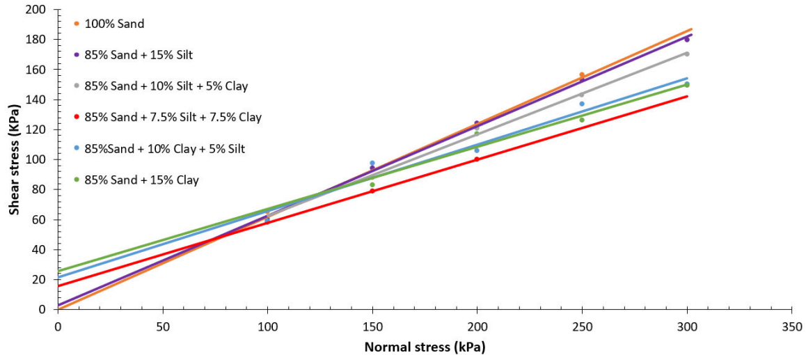
Figure II.6: Mohr-Coulomb Failure envelop for the fine soils
