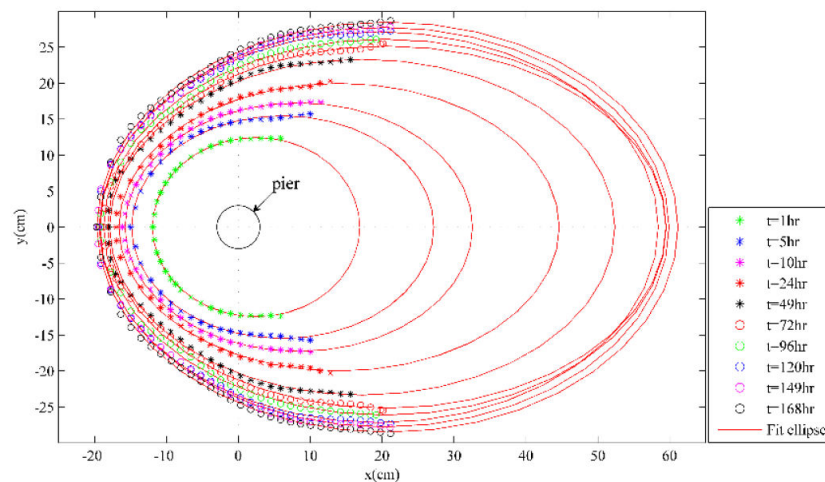
Figure I.14: Elliptical plane shape of the upstream part of the scour hole; Liu et al. 2019 [156]
