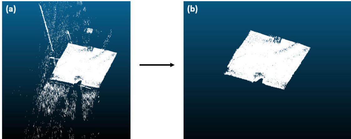
Figure III.8: Cloud cleaning step using Cloud Compare; (a): Cloud before the cleaning step, (b): Cloud after the cleaning step
