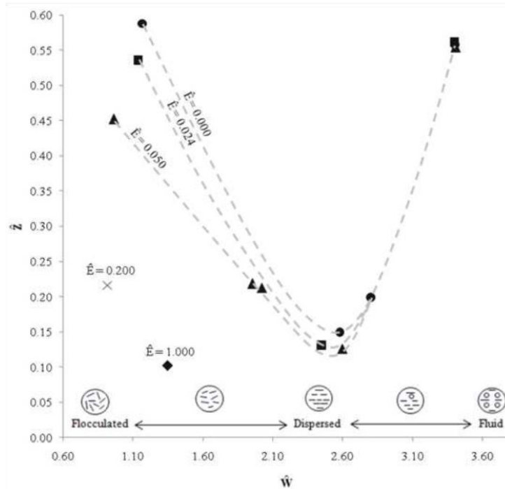
Figure I.29: Variation of the scour depth ratio ( Z (cohesive bed)/ Z (sand)) with dimensionless compaction energy ( E/E_{op} ) and molding water content ( W/W_{op} ); Link et al. 2013 [154]
