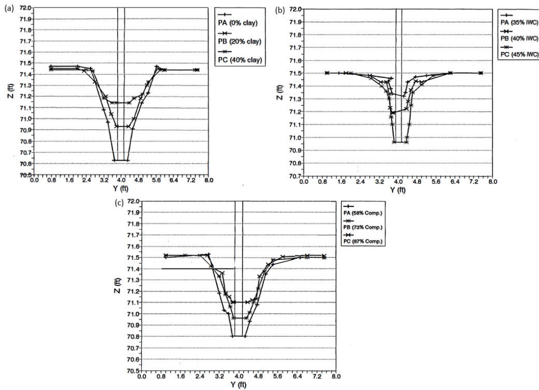
Figure I.19: Transversal scour hole profiles (a) : effect of clay content in cohesive mixtures at Fr = 0.307-0.33 , initial water content (IWC) = 10-12% at the same energy of compaction; (b): effect of initial water content (IWC) in saturated cohesive soils at Fr = 0.367-0.445 , Comp = 86-95\% ; (c): effect of degree of compaction (Comp) in unsaturated cohesive soils at Fr = 0.336-0.369 , IWC = 20\% ; where Fr is the froude number; Molinas and Honsy 1999 [170]
