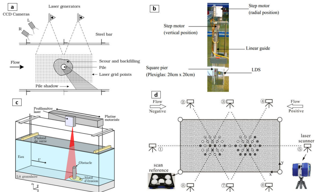
Figure I.8: Experimental techniques for pier scour measurement (a) Stereo-vision measuring scheme adopted by Summer et al. 2013 [236]; (b): Laser Distance Sensor (LDS) system for square pier; Diab 2011 [90]; (c): Profilometer Laser Technique scheme adopted by LaChaussée 2018 [140]; (d): Laser scanner scheme adopted by Ma et al. 2018 [160]
