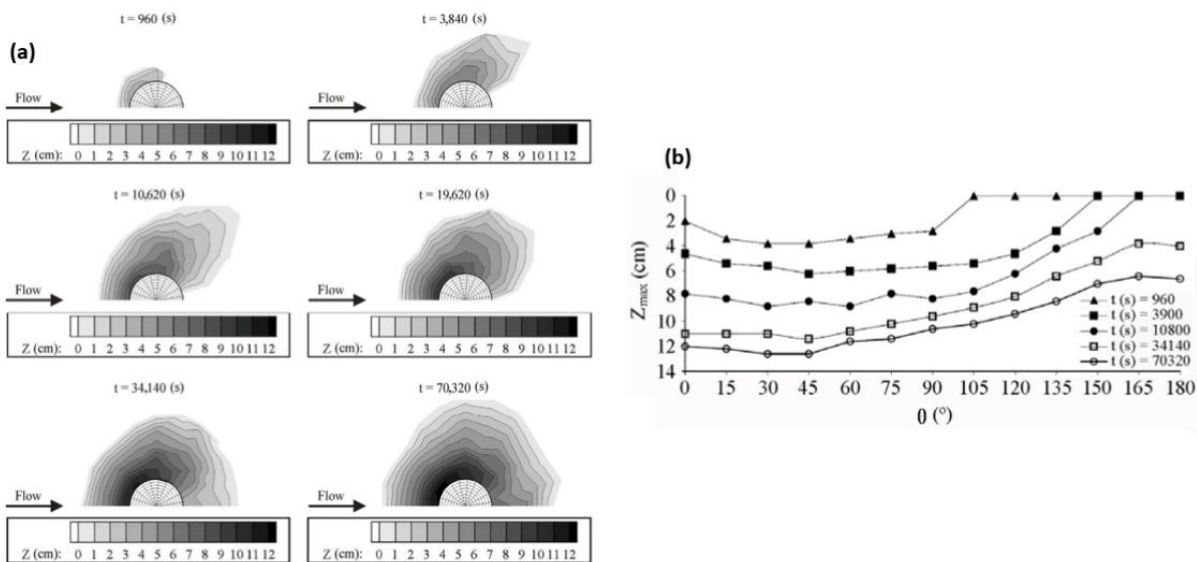
Figure I.16: Dynamic evolution of the scour hole morphology in sand bed, (a):contour plot of the scour hole topography, (b): Scour depth function of azimuth angle; Link et al. 2008 [155]
