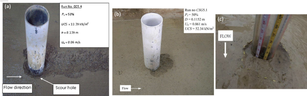
Figure I.30: Scour pattern (a): in Clay-Gravel mixture Kothyari et al. 2014 [131], (b): in Clay-Sand-Gravel mixture Jain et al. 2021 [120]; (c): in natural cohesive soil, U = 0.801 \text{ m/s} , IWC = 38\% Malhader et al. 2021 [161]
