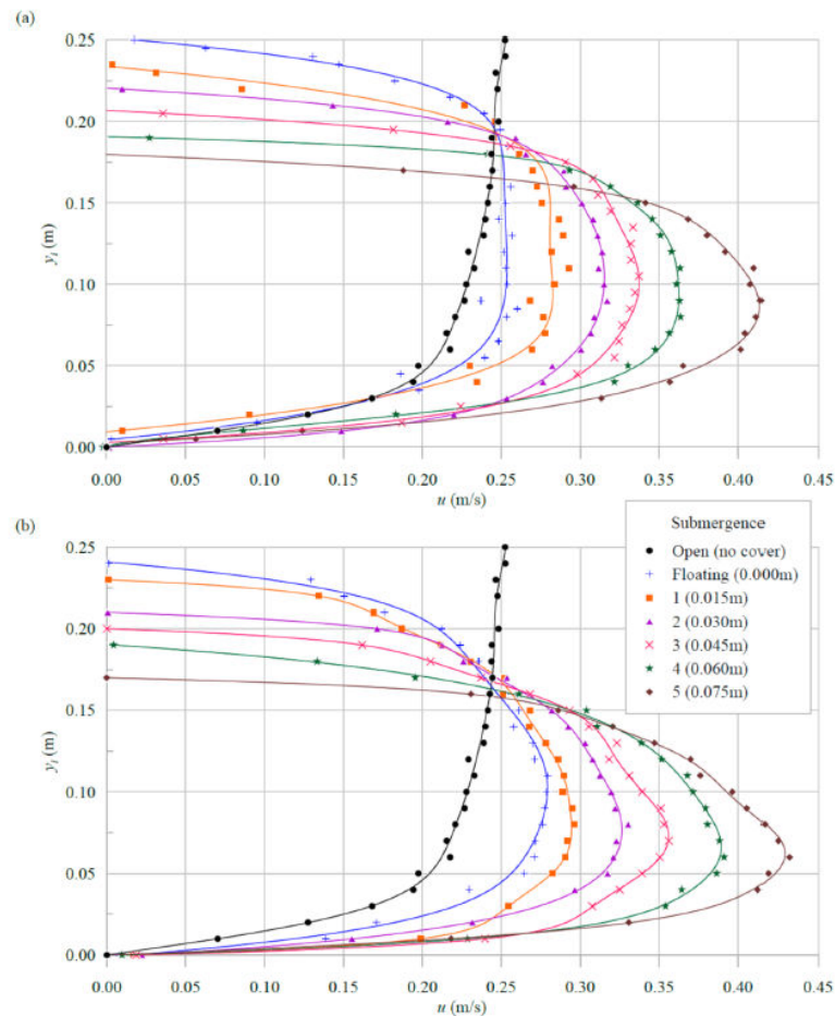
Figure I.9: Velocity profiles for open, floating, and various depth of submerged attached conditions under (a) smooth ice cover and (b) rough ice cover; Valela et al. 2021 [246]
