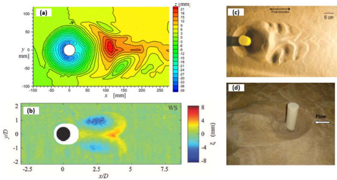
Figure I.17: Scour hole pattern; (a): classical scour hole pattern; Umeda et al. 2008 [244], (b): rabbit ear pattern; Lachausée et al. 2018 [141], (c): Succession of sedimentary patterns downstream of a cylinder; Sarkar et al. 2016 [213], (d): Scour hole pattern in live bed scour; Zhao et al. 2010 [265]
