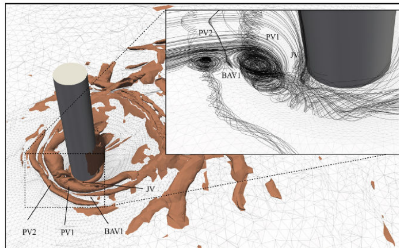
Figure I.4: Numerical simulation showing necklace vortices inside the scour hole for live bed scour regime ( Re_b=46000 ); JV: Joint Vortex, PV: Primary Vortex, BAV: Bottom-Attached Vortex, SV: Secondary Vortex; Zhang et al. 2020 [264]
