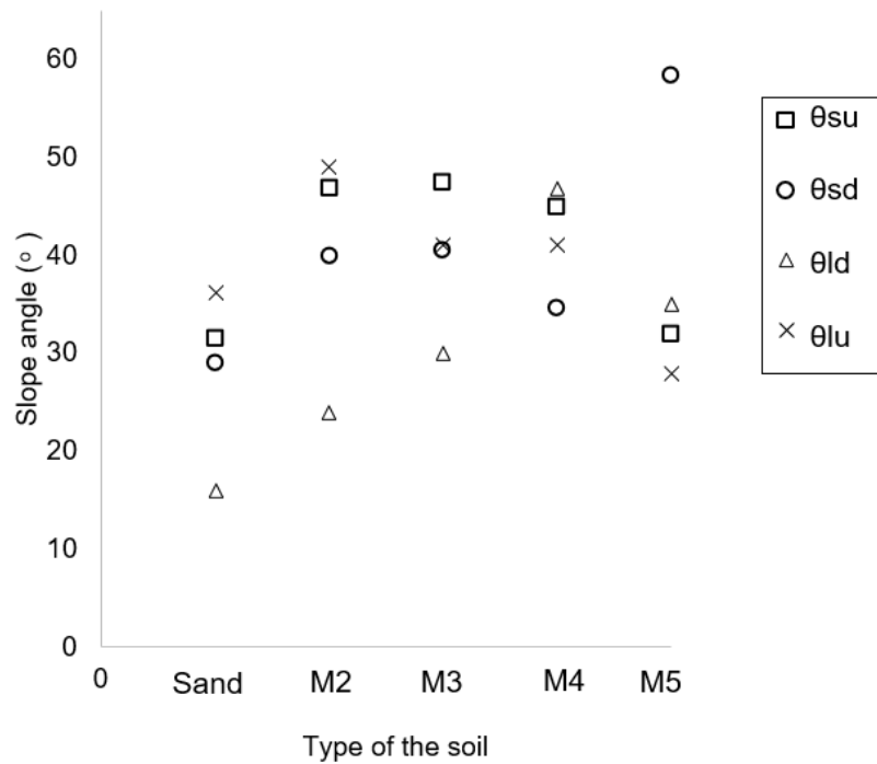
Figure IV.8: Slope of the scour hole at the end of the tests (360 min) as a function of the type of the soil; \theta_{lu} , \theta_{su} , \theta_{ld} , \theta_{sd} are the longitudinal slope upstream, the average side slope upstream, the longitudinal slope downstream and the average side slope downstream respectively and M2, M3, M4 and M5 are 85% sand +10 % silt +5 % clay, 85% sand +7.5 % silt +7.5 % clay, 85% sand +5 % silt +10 % clay and 85% sand +15 % clay respectively
