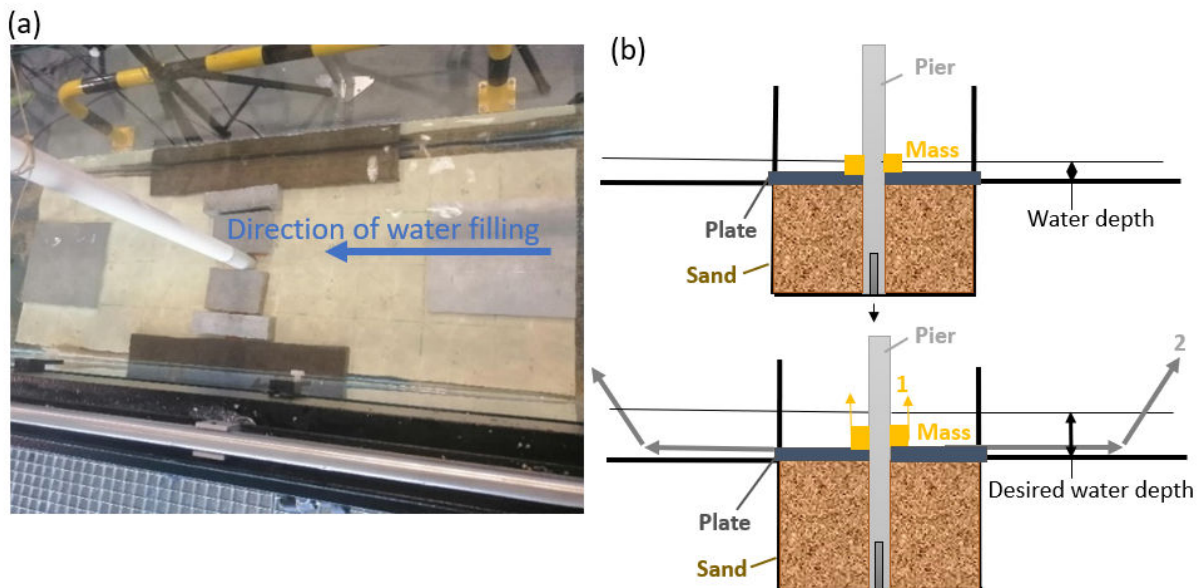
Figure II.21: Water filling procedure for medium sand, (a): photograph taken during the water filling step, (b): Illustration of the applied methodology
