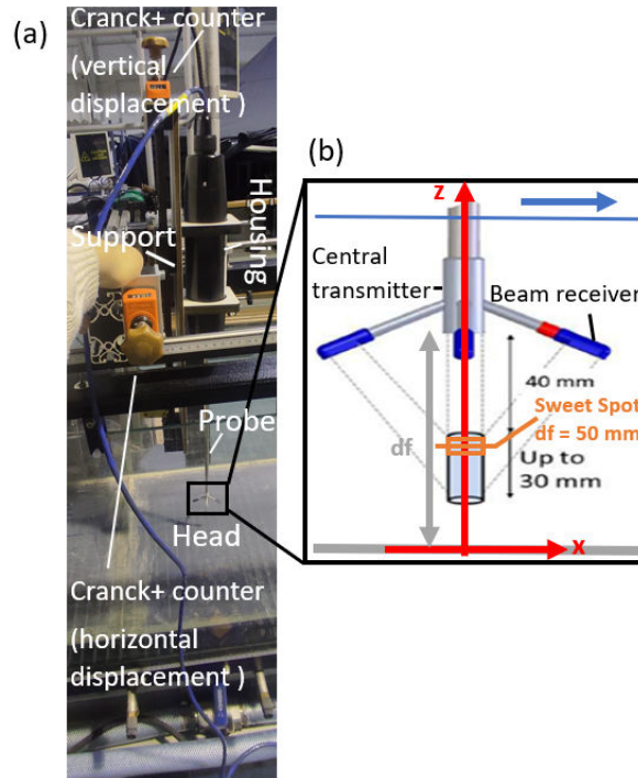
Figure II.11: Nortek Vectrino Profiler, (a): Installation of the Vectrino on the flume, (b): notation and sampling volume after [183], the direction of the flow is indicated by blue arrows
