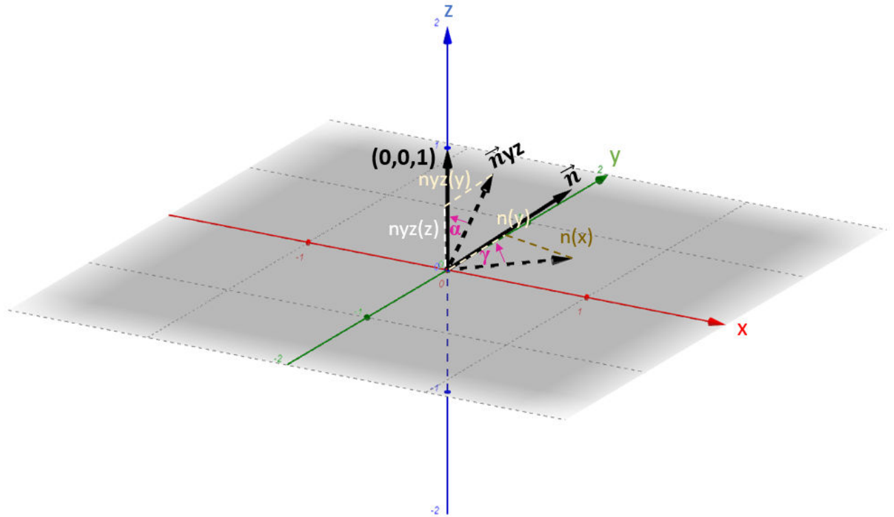
Figure III.6: Rotation angles, \gamma is the angle used in the rotation matrix R_z and \alpha is the angle used in the rotation matrix R_x ; n(x) and n(y) are the components of the unit vector n along the x and y axes, respectively, nyz is the component of vector n in the (yz) plane, nyz(y) and nyz(z) are the components of the vector nyz along the y and z axes, respectively
