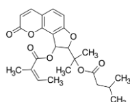
2'-angeloyl-3'-isovaleryl vaginate
