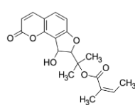
vaginidiol-O-angelate
