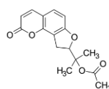
columbianetin acetate
