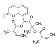
archangelicin
