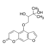
oxypeucedanin hydrate
