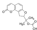
columbianetin acetate
