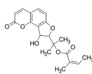
vaginidiol-O-angelate
