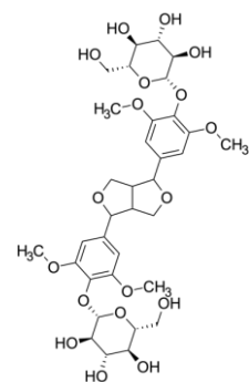
syringaresinol 4,4'-di-O-glucoside
