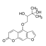
oxypeucedanin hydrate
