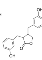
enterolactone
