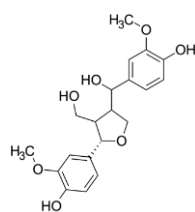
7-hydroxylariciresinol
