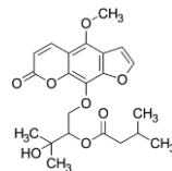
byakangelicin-2'-O-isovalerate
