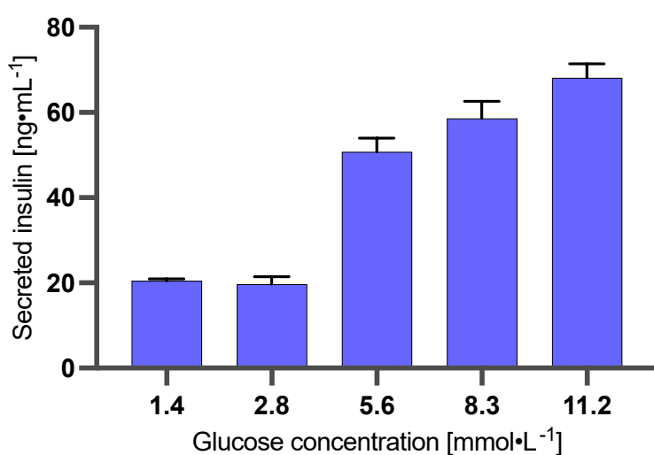
Figure 27. Glucose effect on insulin secretion.
