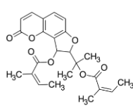
archangelicin
