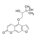
oxypeucedanin hydrate
