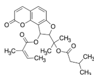
2'-angeloyl-3'-isovaleryl vaginate
