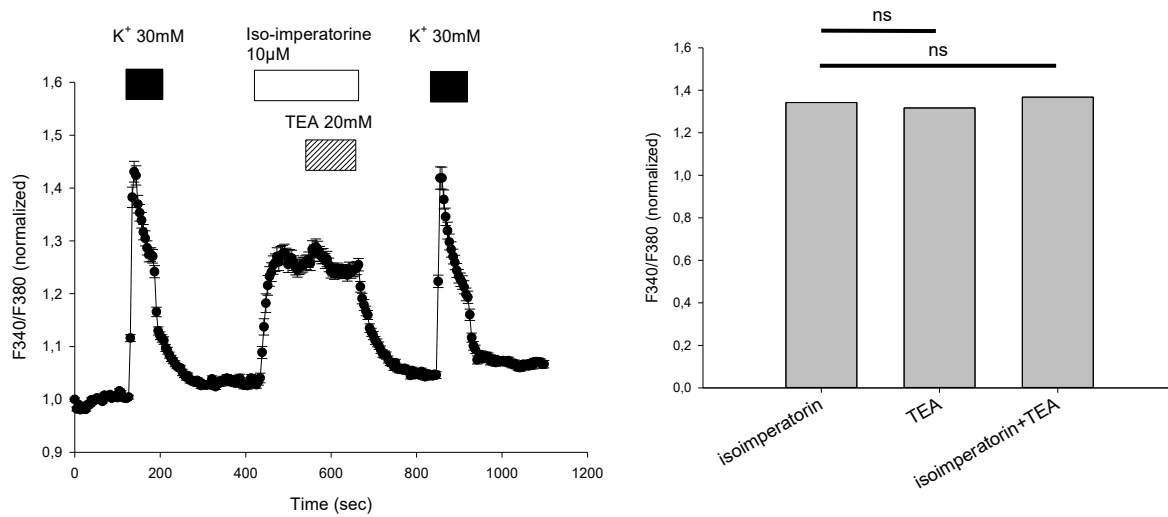
Figure 51. Isoimperatorin effect on intracellular calcium levels in the presence of VGKC blocker (TEA).
