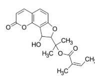
vaginidiol-O-angelate
