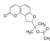
columbianetin acetate
