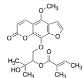
byakangelicin-2'-O-angelate
