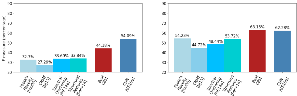
Figure 3.15 – Segmentation results of the best CBM algorithm, compared to the other State-of-the-Art algorithms. Results are computed on the SALAMI dataset.
