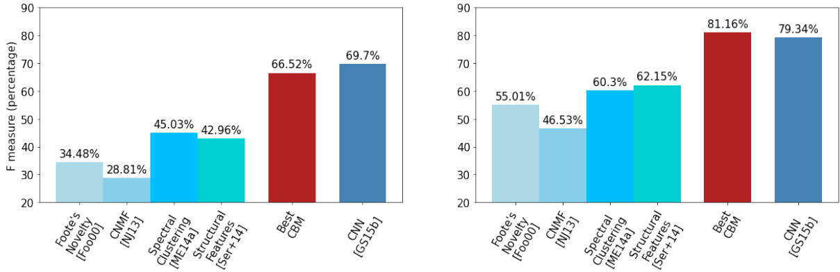
Figure 3.14 – Segmentation results of the best CBM algorithm, compared to the other State-of-the-Art algorithms. Results are computed on the RWC Pop dataset.
