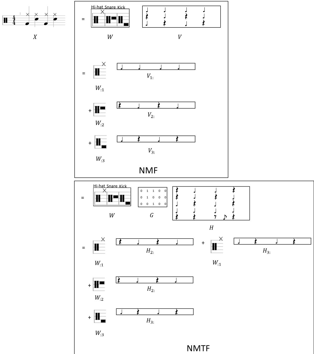
Figure 4.7 – Drum pattern from Figure 4.6, decomposed in both NMF and NMTF models. Matrix H is composed of 5 different barwise rhythmic templates, but only 2 are actually used ( H_2 and H_3 ), presenting H as a dictionary of rhythmic patterns. This is useful in the interpretation of NTD, as matrices W and H can be interpreted as dictionaries of pitch-related and duration-related information (at barscale) in the song.
