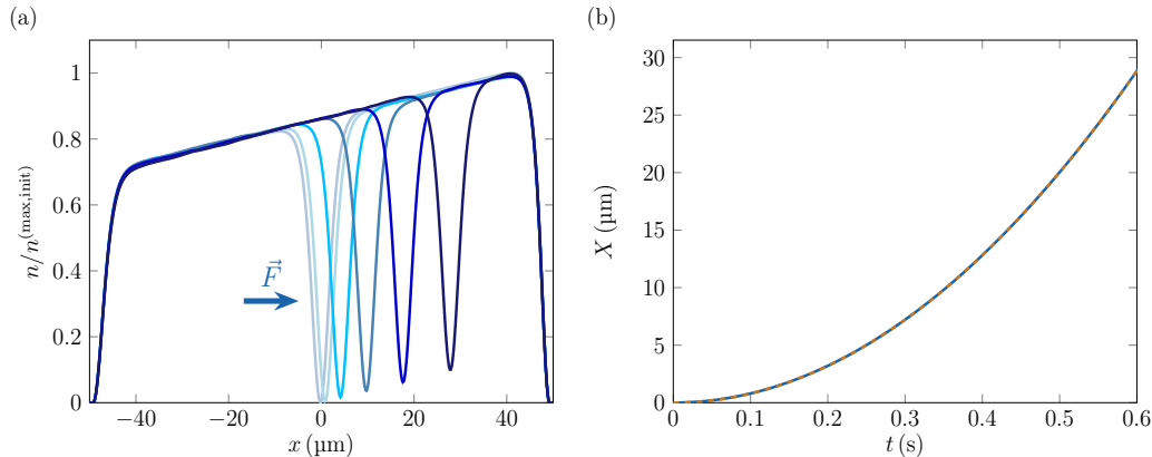
FIGURE E.2: Numerical simulation of a dark soliton under a constant force directed along +\vec{x} . The GP simulation is run for a positive scattering length a = 2.63a_B , N = 10000 atoms, a magnetic force g_F \mu_B b \simeq 3 \times 10^{-5} mg ( g is the gravity acceleration here). The force is applied on a condensate already at equilibrium with the force. (a): Profiles every \Delta t = 0.3 s. The darker the color the longer the time. The background density is tilted due to the force. (b): The position of the density hole of the wavepacket as a function of time is represented with a blue solid line. The orange dashed line is the prediction (E.10).
