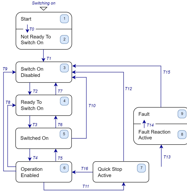
Figure 34: Servo drive FSM from IEC 61800 standard
