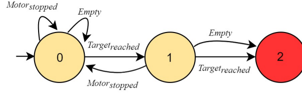
Figure 29: FSM generated by LTL 3 Tools for the formula \square(Target_{reached} \rightarrow \circ Motor_{stopped})
