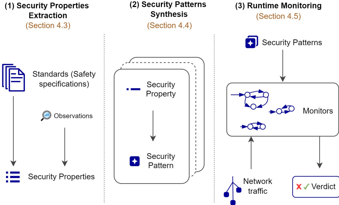
Figure 24: Overview of our approach
