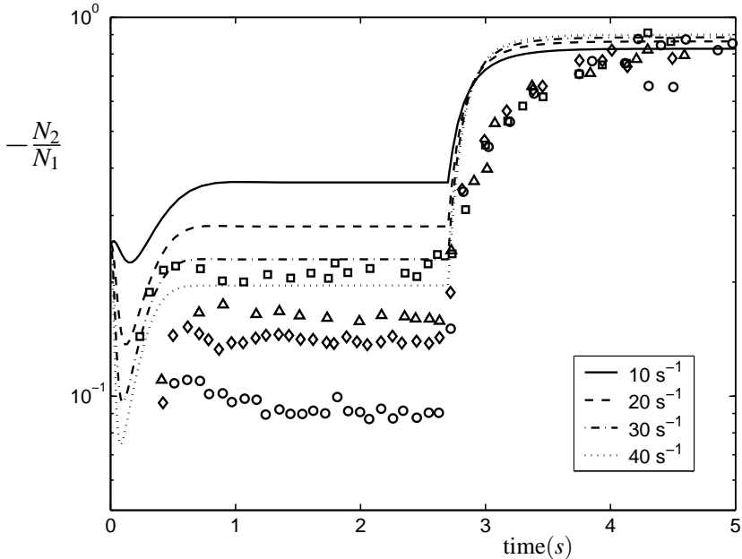
Figure 5.8: Transient first normal stress ratio as a function of time for the proposed model with \alpha = 1 . Corresponding experimental data taken from [64].
