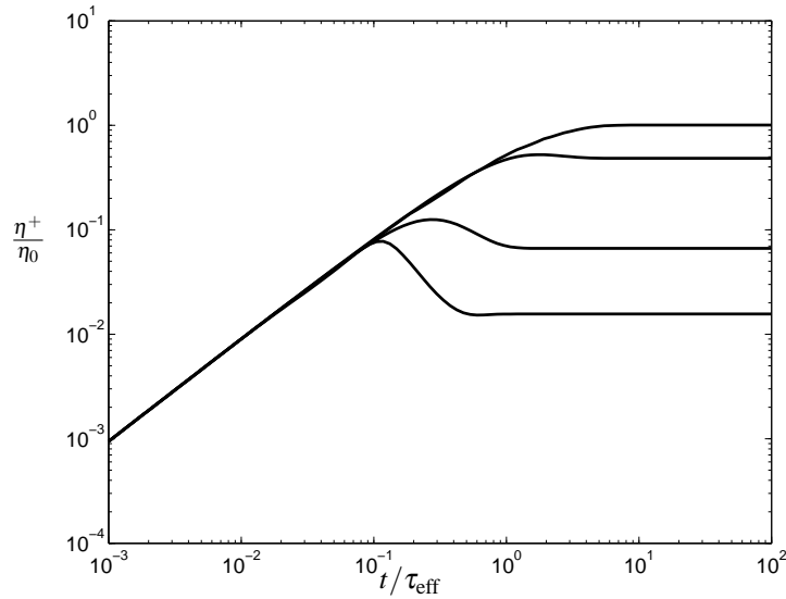
Figure 3.5: Transient shear viscosity for four different Deborah numbers. From the top, the respective Deborah numbers are 0.01, 1, 10 and 100. The finite extensibility parameter b is set to 100 and \tau_d/\tau_r = 30 .
