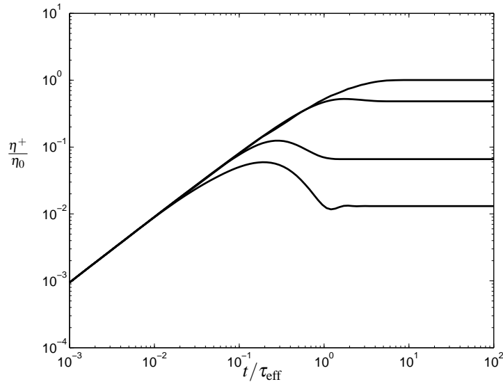
Figure 3.3: Transient shear viscosity for four different Deborah numbers. From the top, the respective Deborah numbers are 0.01, 1, 10 and 100. Finite extensibility has been neglected and \tau_d/\tau_r = 30 .
