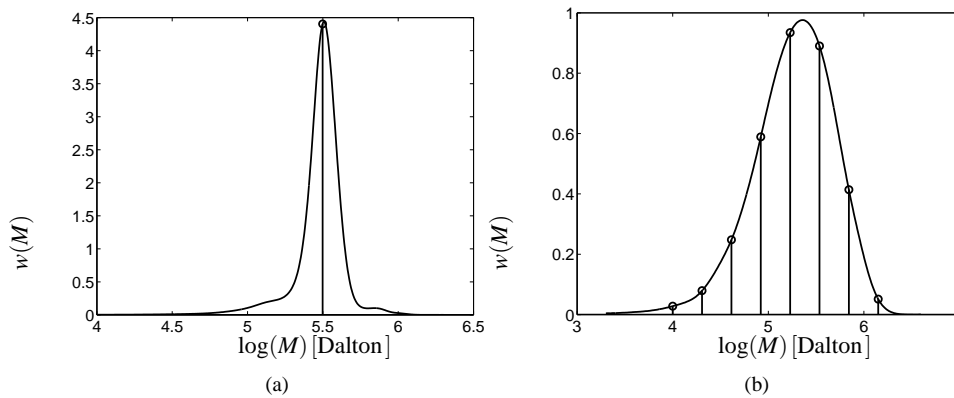
Figure 4.4: Molecular weight distributions of PS1 (a) and PS2 (b) and their discrete approximations.
